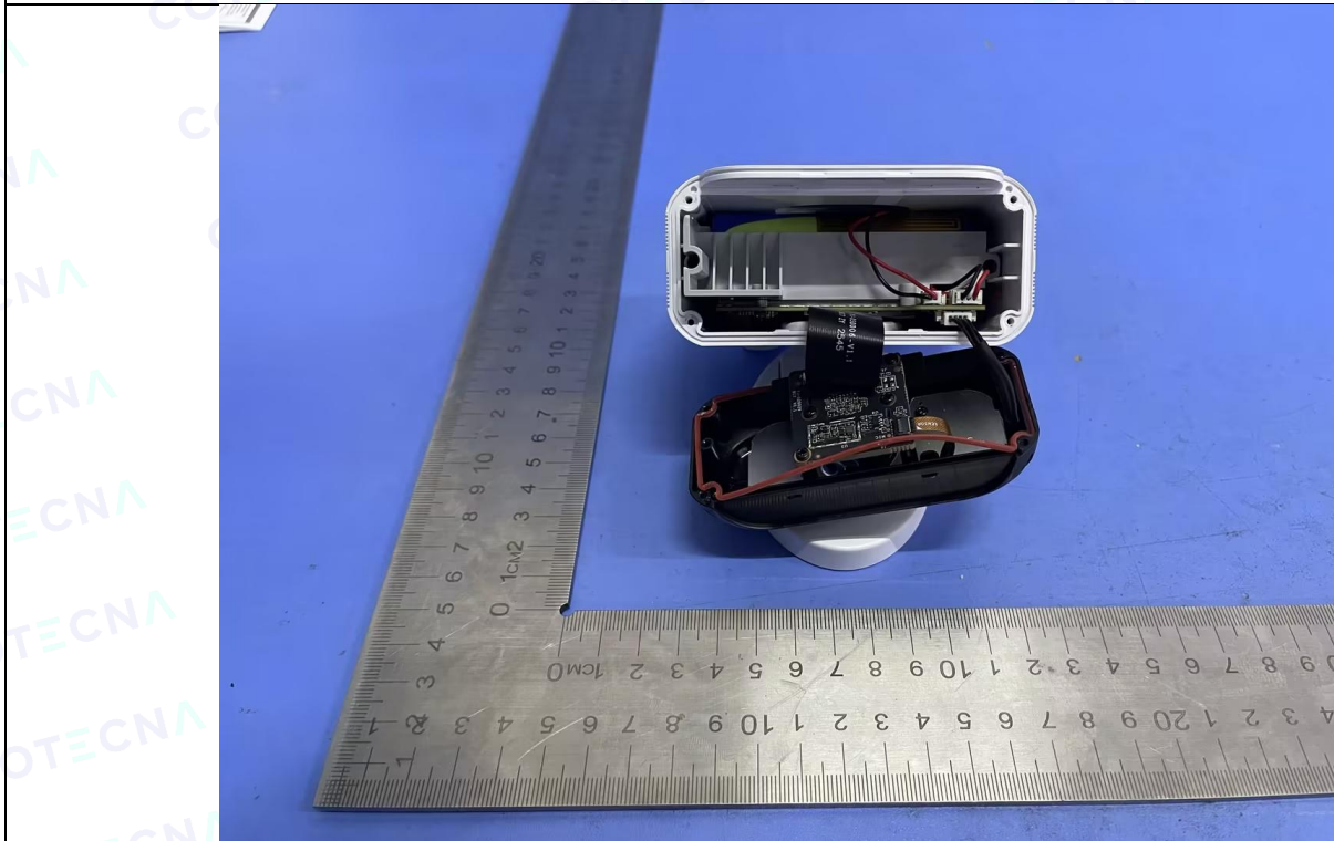
Photo 8 Internal of EUT
