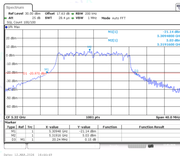
11A-Ant1-5320
