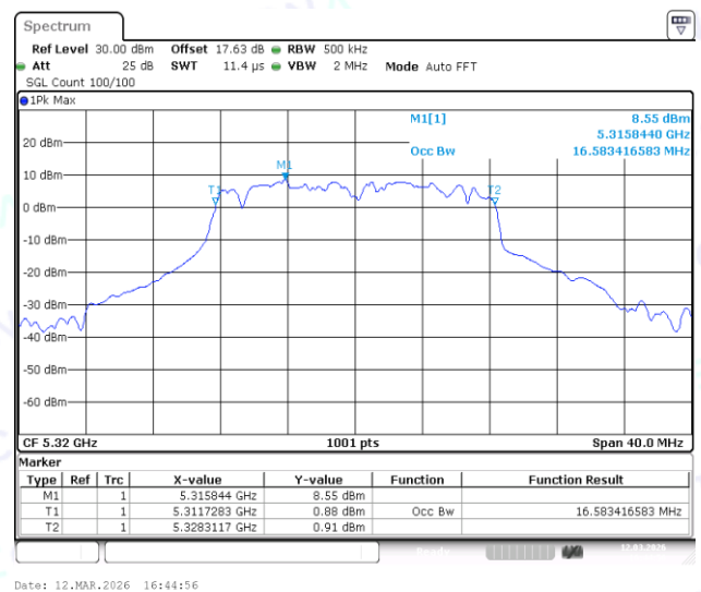
11A-Ant1-5320
