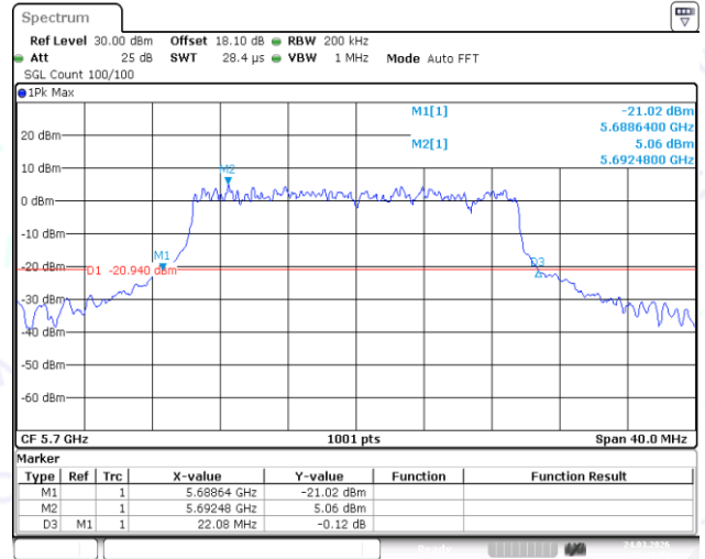
11AX20SISO-Ant1-5700
