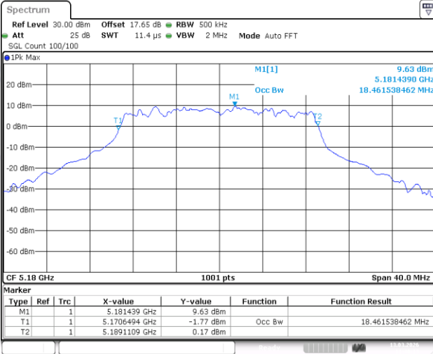
11N20SISO-Ant1-5180
