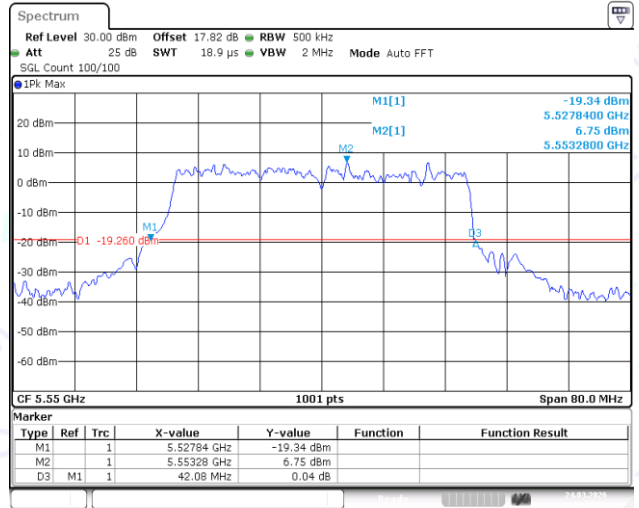
11AX40SISO-Ant1-5550
