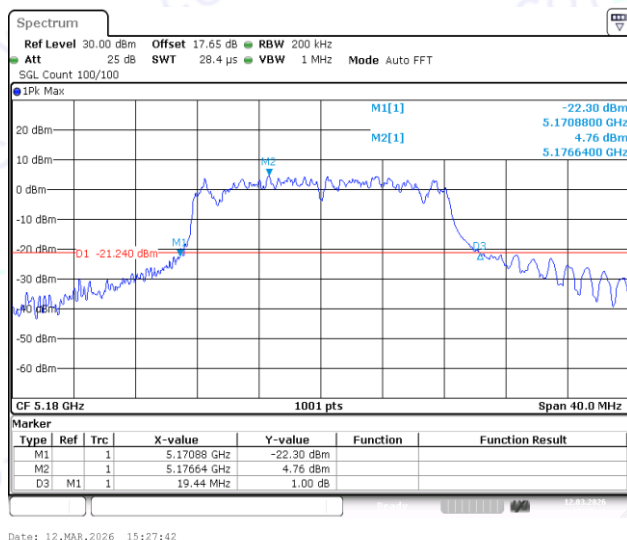
11A-Ant1-5180
