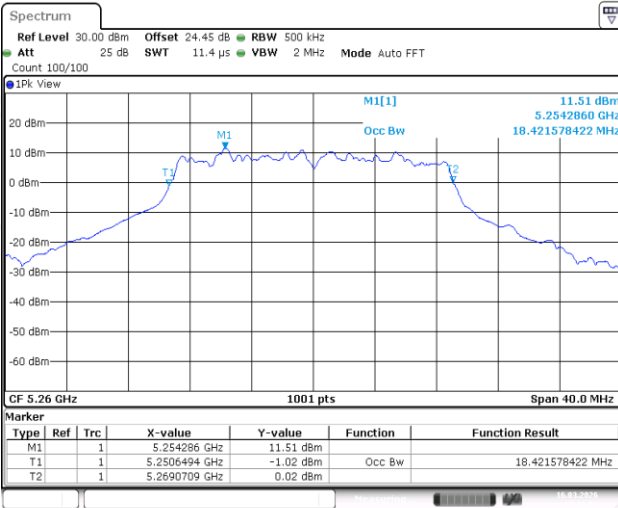
11AC20SISO-Ant1-5260
