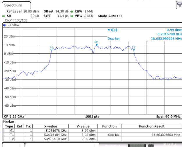
11N40SISO-Ant1-5230
