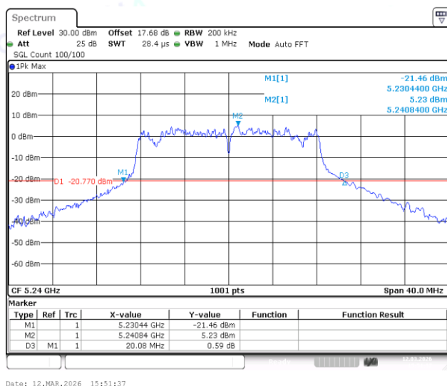
11A-Ant1-5240
