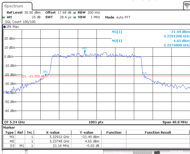
11AX20SISO-Ant1-5240
