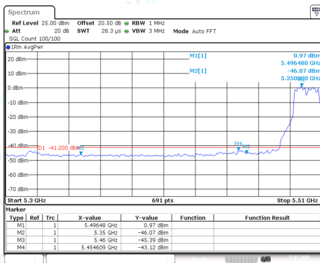
11A-Ant1-5500-PASS
