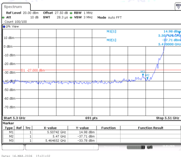
11AC20SISO-Ant1-5500-PASS
