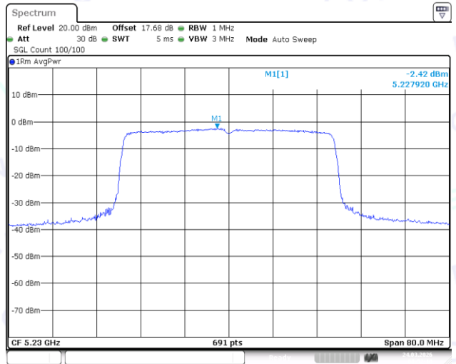
11AX40SISO-Ant1-5230-PASS
