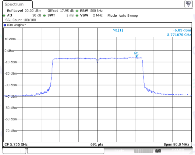
11AX40SISO-Ant1-5755-PASS
