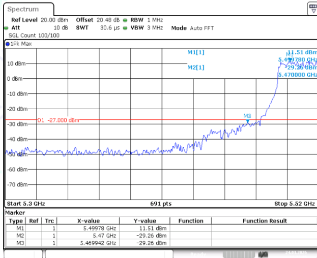
11AC40SISO-Ant1-5510-PASS
