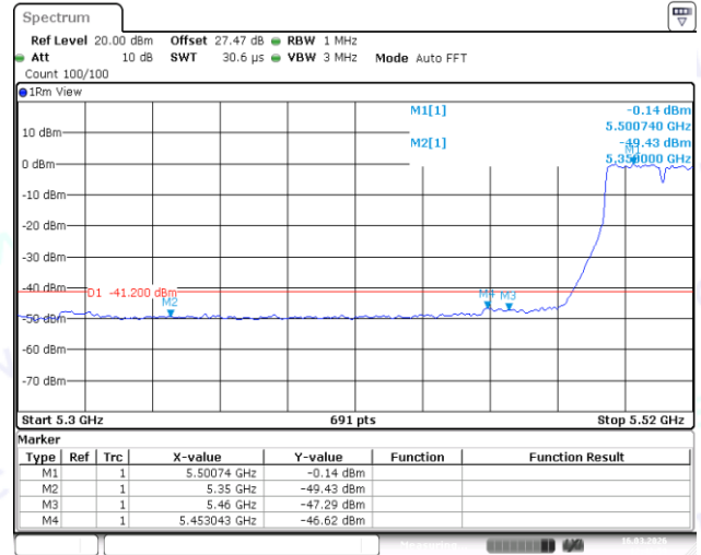
11N40SISO-Ant1-5510-PASS
