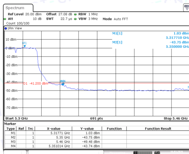
11N40SISO-Ant1-5310-PASS
