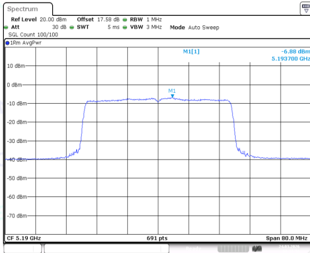
11AX40SISO-Ant1-5190-PASS
