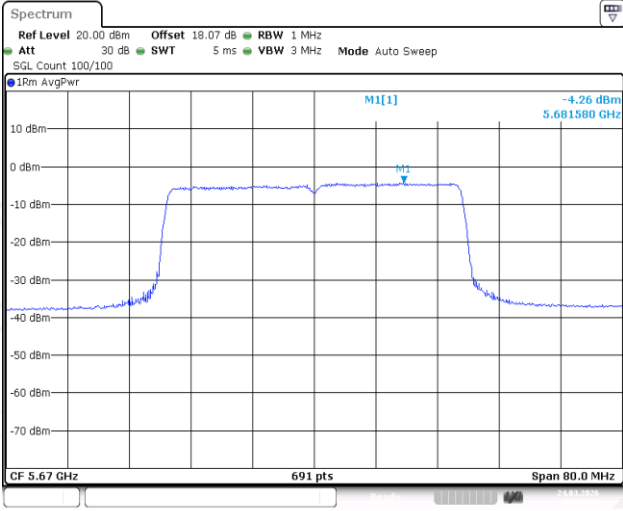
11AX40SISO-Ant1-5670-PASS
