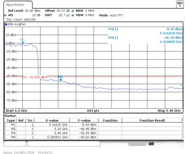
11AX40SISO-Ant1-5310-PASS
