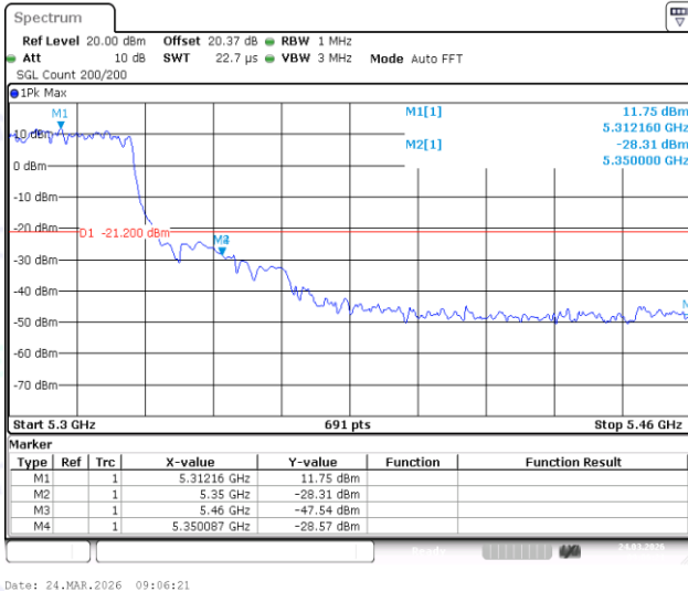
11AX40SISO-Ant1-5310-PASS
