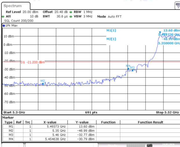
11AC40SISO-Ant1-5310-PASS
