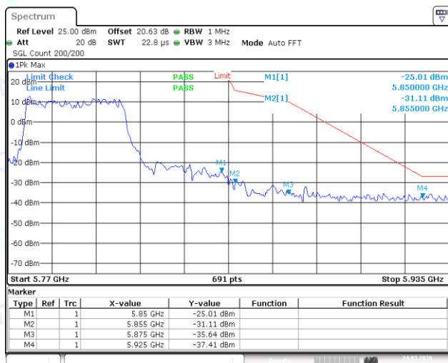
11AC40SISO-Ant1-5795-PASS
