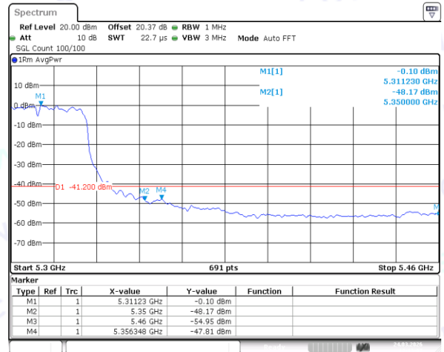
11AC40SISO-Ant1-5310-PASS
