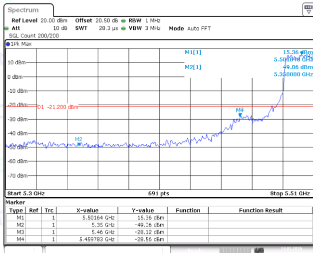
11AX20SISO-Ant1-5500-PASS
