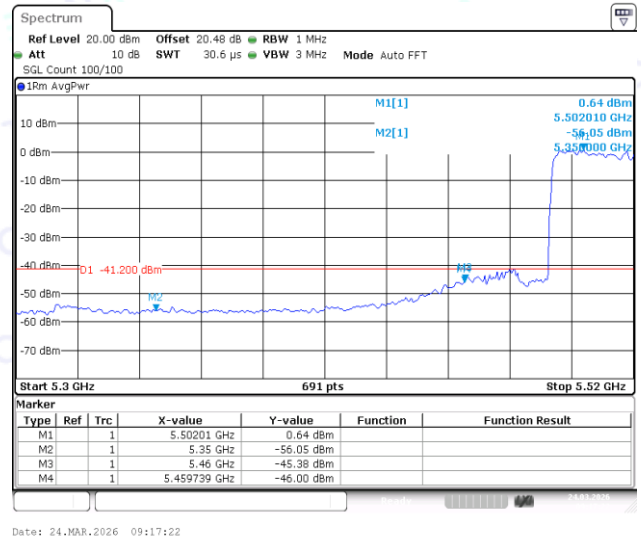
11AX40SISO-Ant1-5510-PASS
