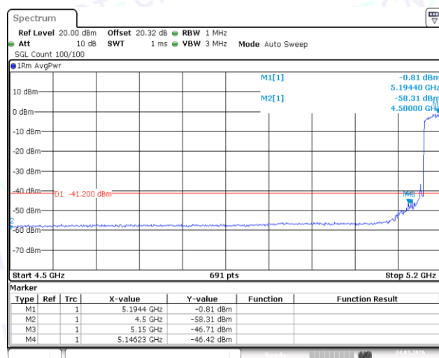
11AX40SISO-Ant1-5190-PASS
