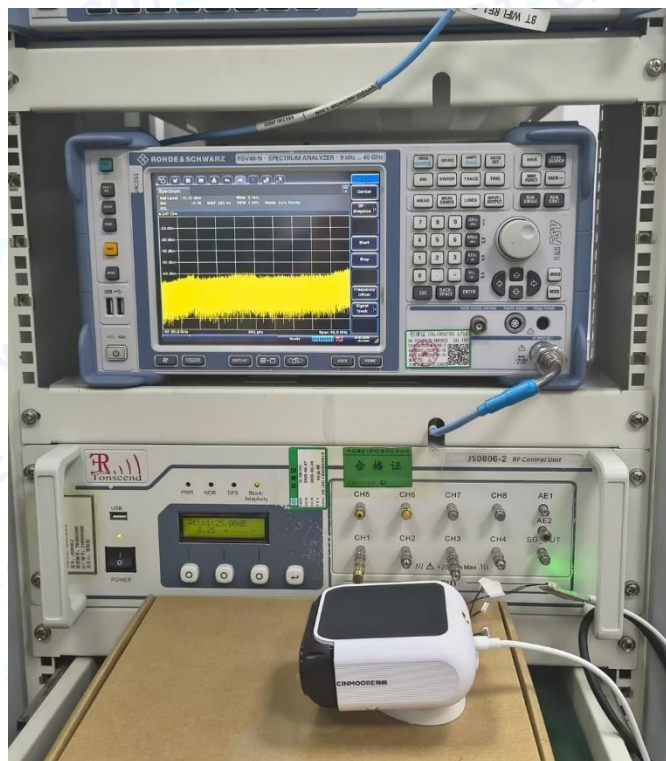
Photo of Setup for Conducted Measurements
