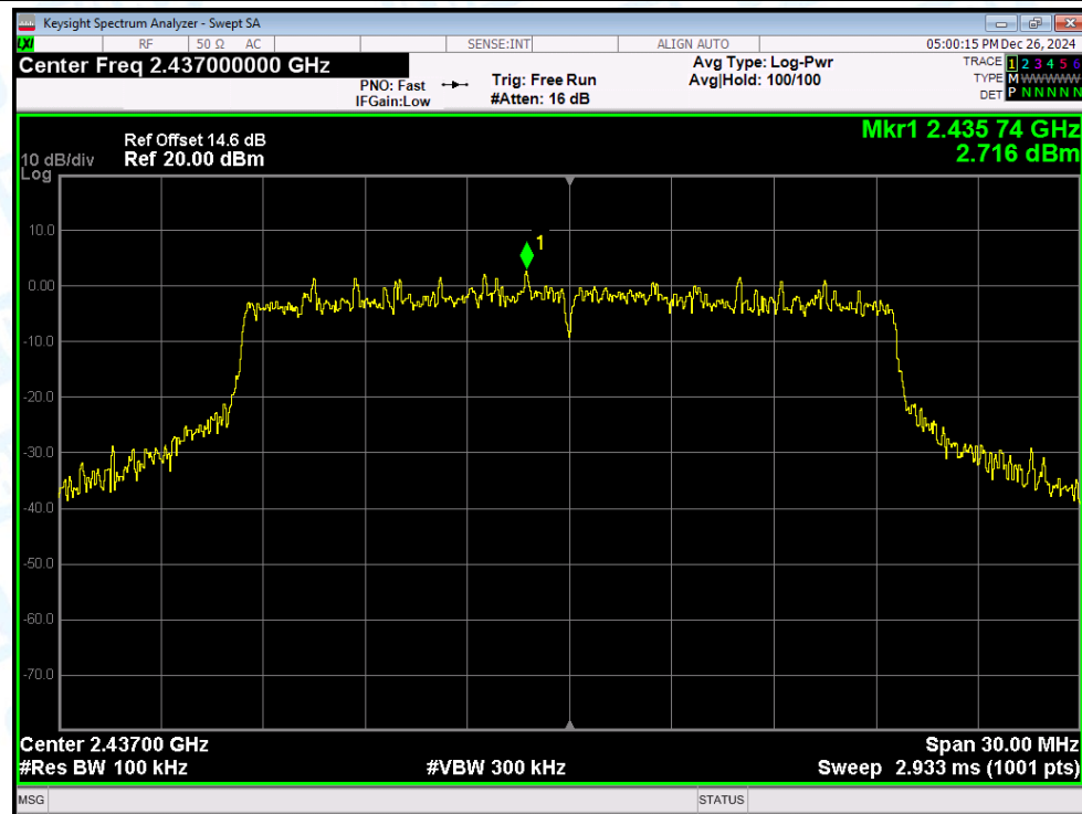
Tx. Spurious NVNT ax(VHT20) 2437MHz Ant1 Emission
