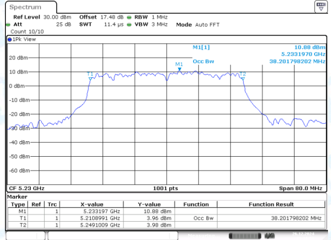
11AX40SISO-Ant1-5230
