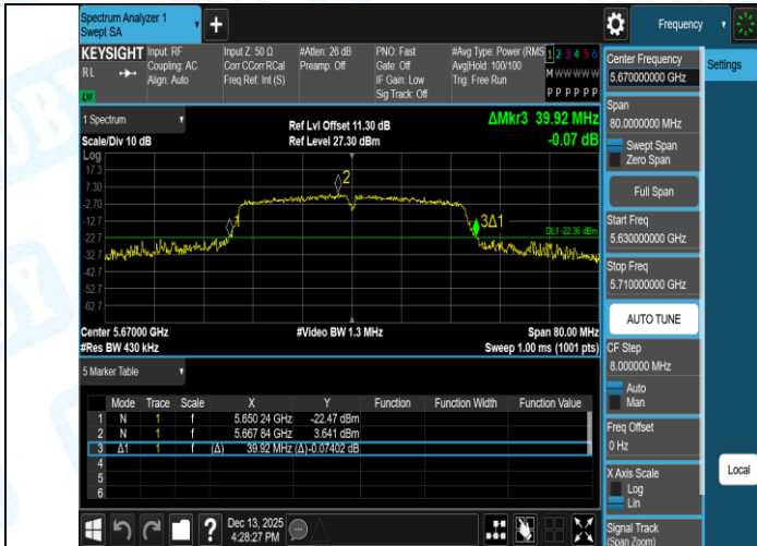
11N40SISO-Ant1-5670
