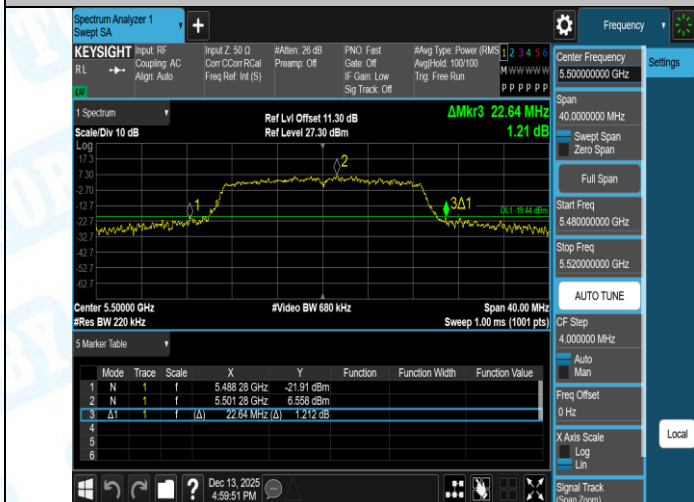
11AC20SISO-Ant1-5500
