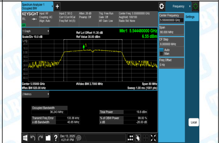
11N40SISO-Ant1-5550
