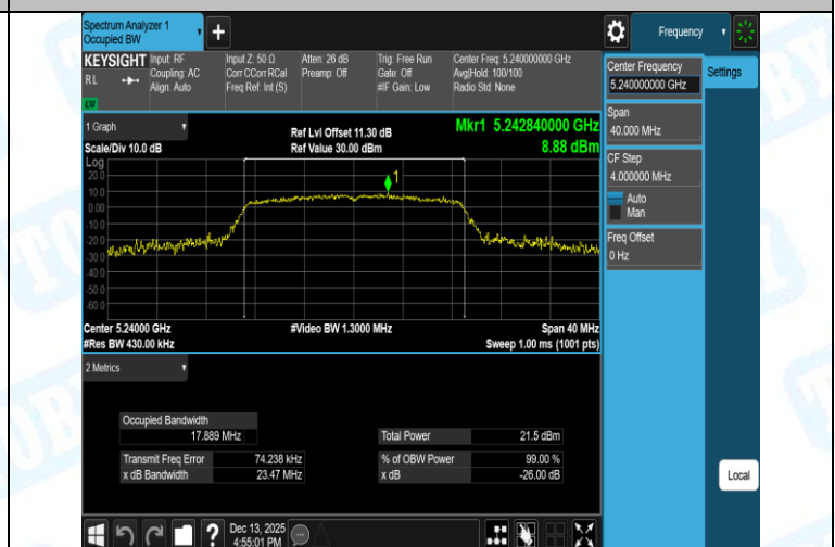
11AC20SISO-Ant1-5240
