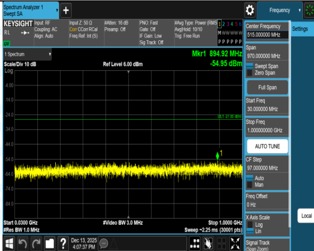
11N40SISO-Ant1-5270-30~1000-PASS
