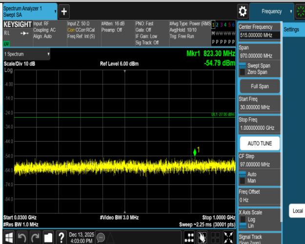
11N40SISO-Ant1-5230-30~1000-PASS
