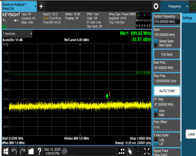
11N40SISO-Ant1-5190-30~1000-PASS
