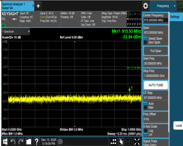
11AC40SISO-Ant1-5310-30~1000-PASS
