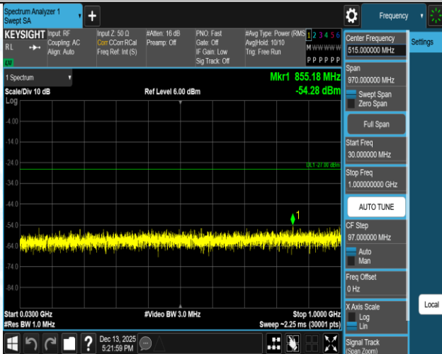
11AC40SISO-Ant1-5550-30~1000-PASS
