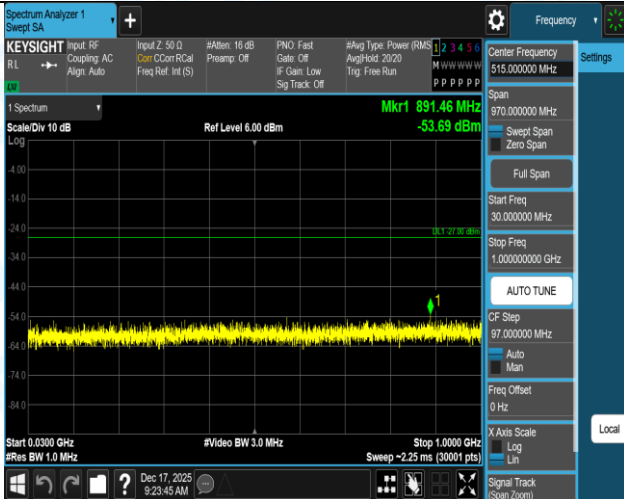
11AX20SISO-Ant1-5745-30~1000-PASS
