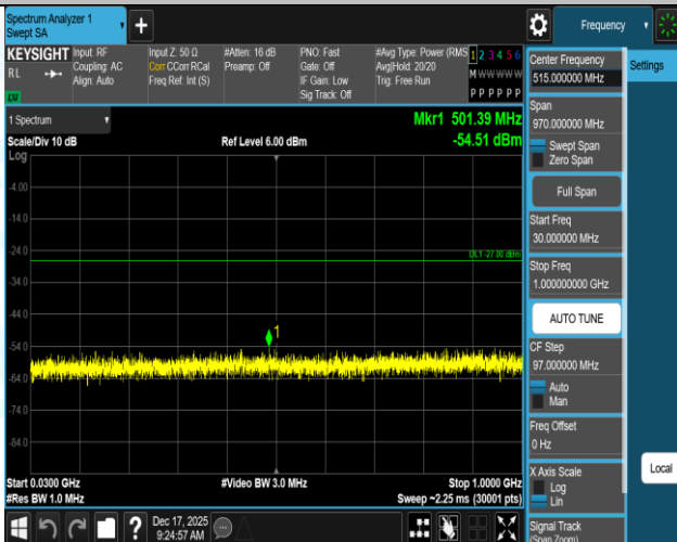
11AX20SISO-Ant1-5785-30~1000-PASS
