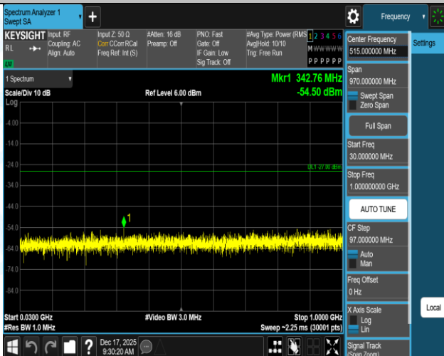
11AX40SISO-Ant1-5230-30~1000-PASS
