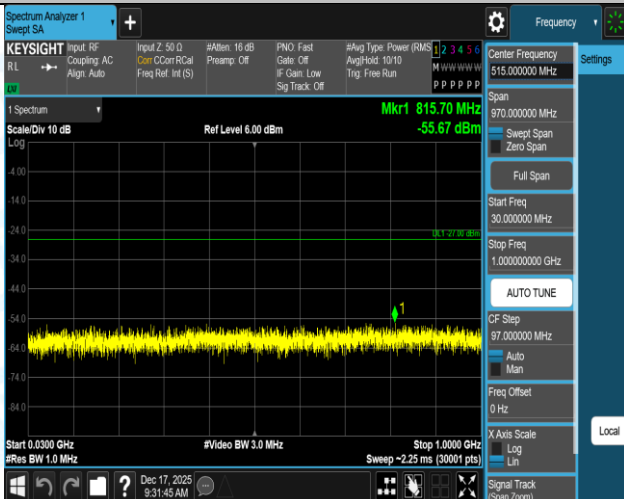
11AX40SISO-Ant1-5270-30~1000-PASS
