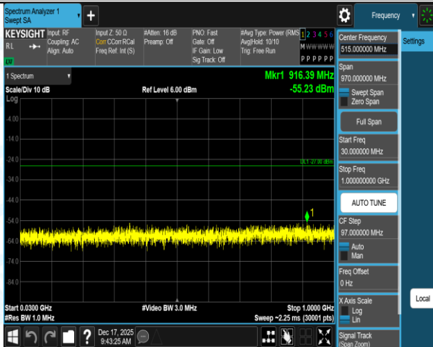
11AX40SISO-Ant1-5550-30~1000-PASS
