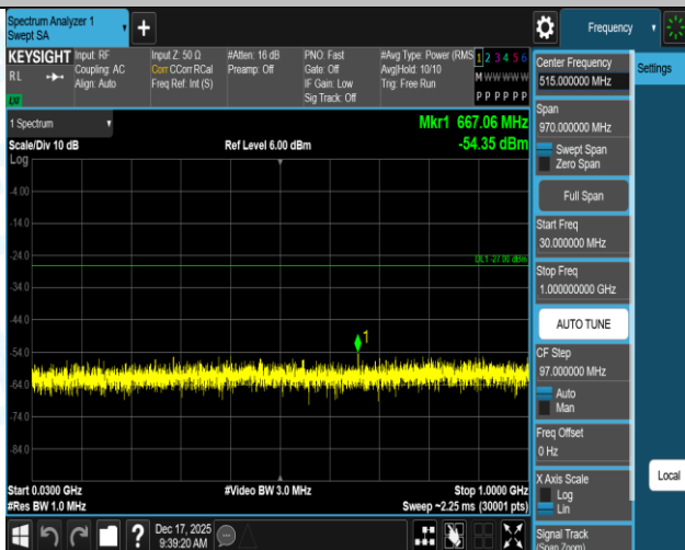
11AX40SISO-Ant1-5510-30~1000-PASS
