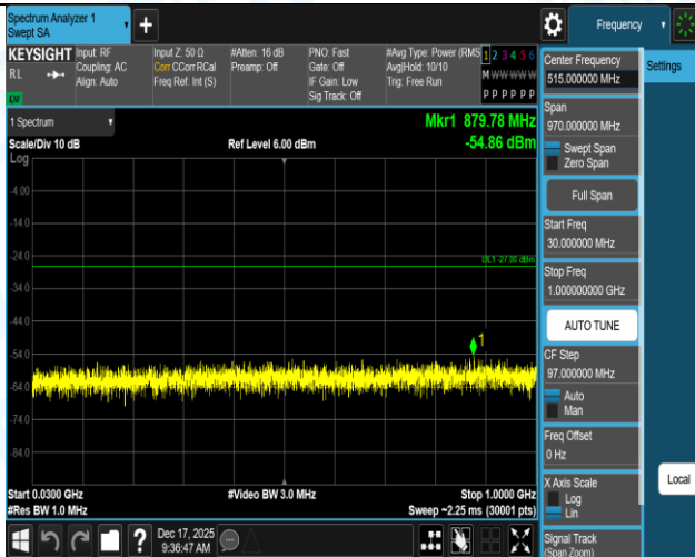
11AX40SISO-Ant1-5310-30~1000-PASS
