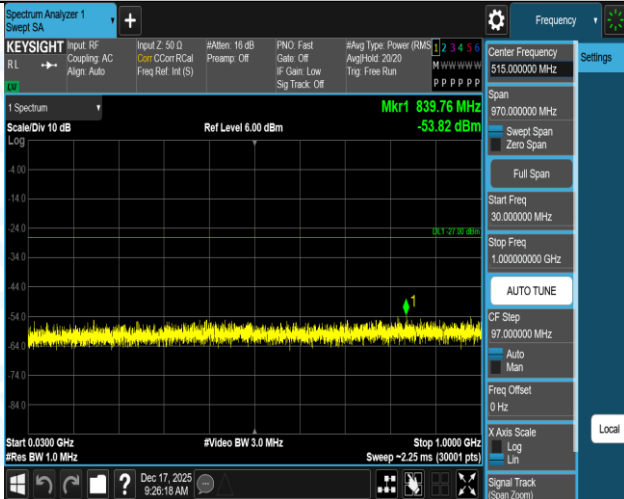
11AX20SISO-Ant1-5825-30~1000-PASS
