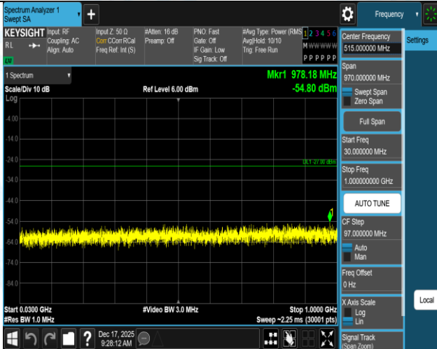
11AX40SISO-Ant1-5190-30~1000-PASS
