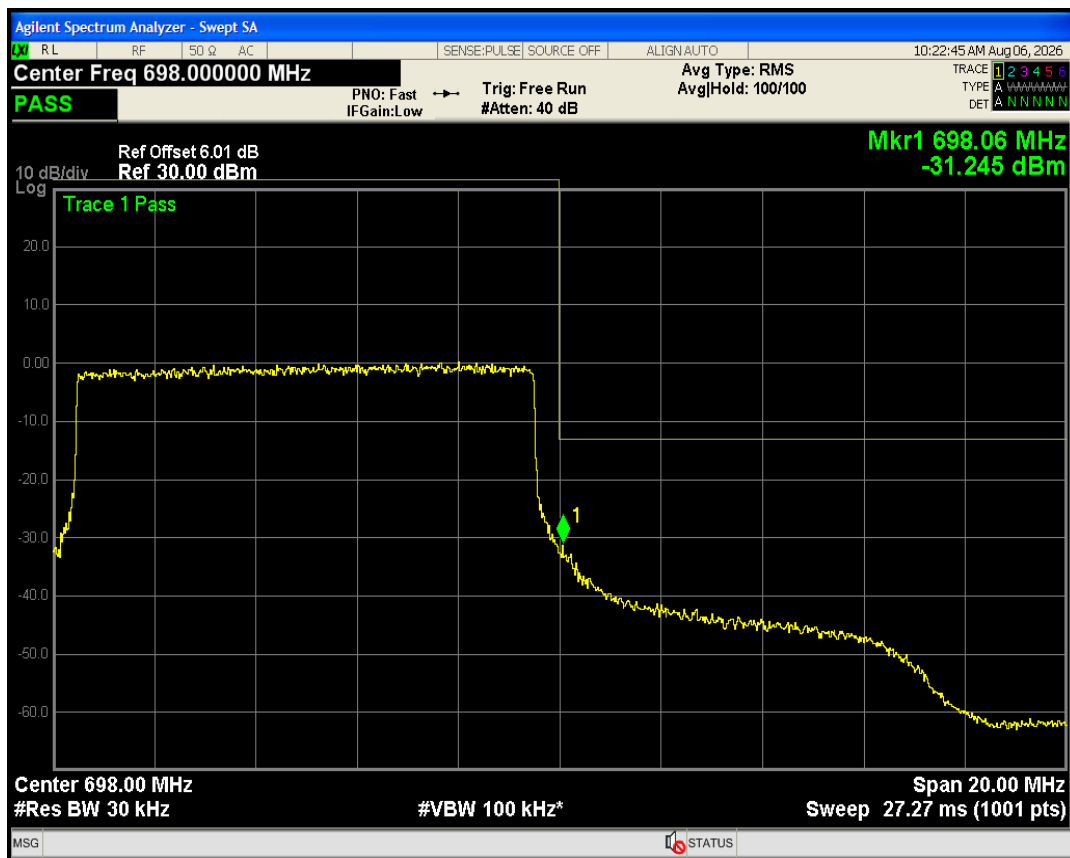
Band71 QAM16 BW=10MHz Channel=133422 RB Size=27 Position=#0
