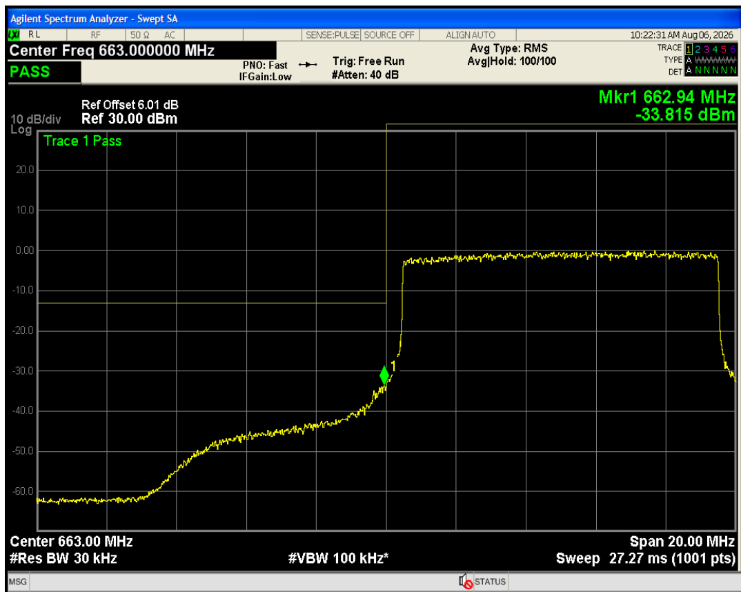
Band71 QAM16 BW=10MHz Channel=133172 RB Size=27 Position=#0
