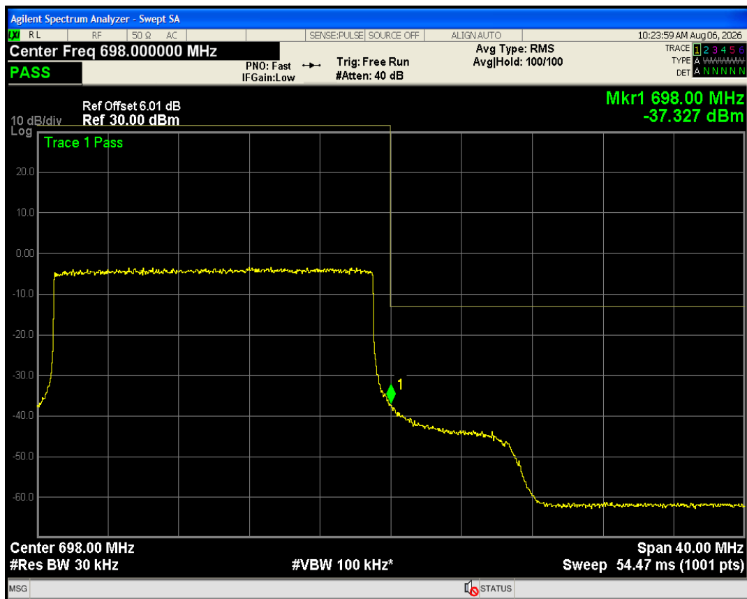
Band71 QAM16 BW=20MHz Channel=133372 RB Size=27 Position=#0
