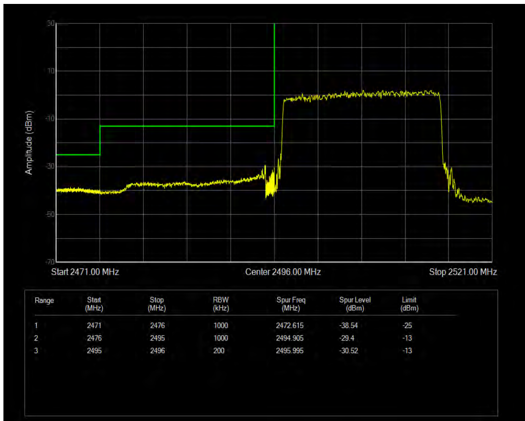
Band41 QAM16 BW=20MHz Channel=39750 RB Size=27 Position=#0
