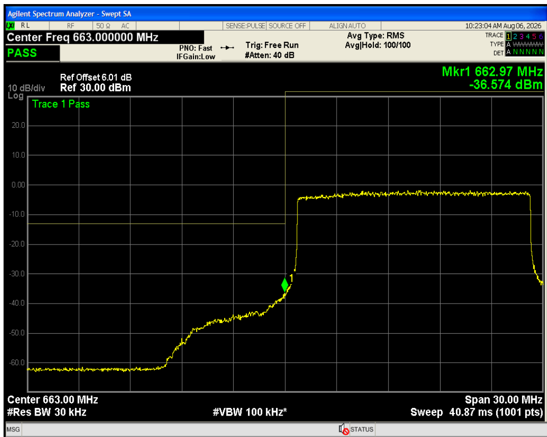
Band71 QAM16 BW=15MHz Channel=133197 RB Size=27 Position=#0
