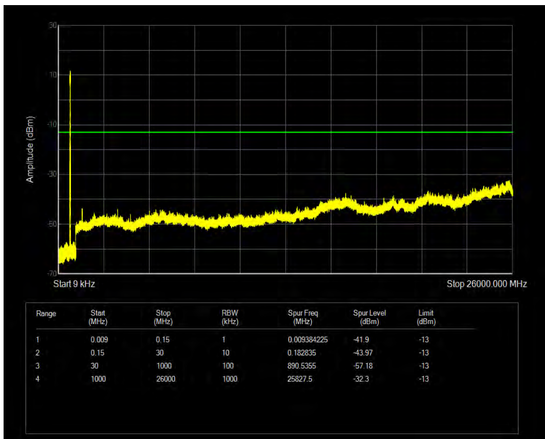
Band71 QAM16 BW=20MHz Channel=133372 RB Size=27 Position=#0
