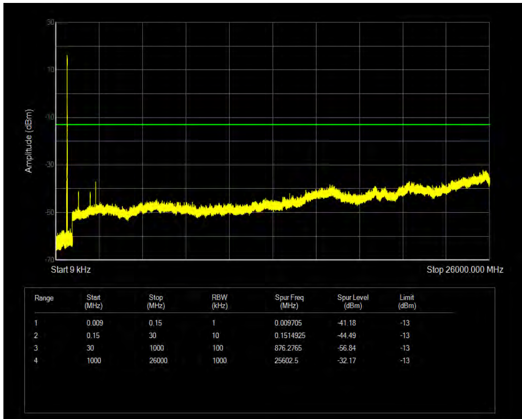
Band71 QAM16 BW=15MHz Channel=133197 RB Size=27 Position=#0
