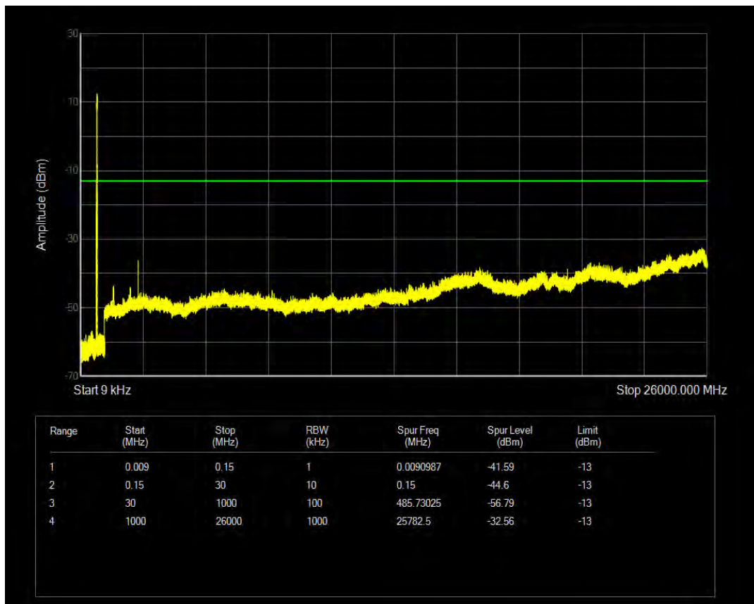
Band71 QAM16 BW=15MHz Channel=133397 RB Size=27 Position=#0
