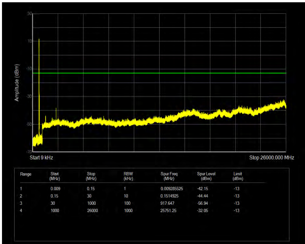
Band71 QAM16 BW=20MHz Channel=133222 RB Size=27 Position=#0
