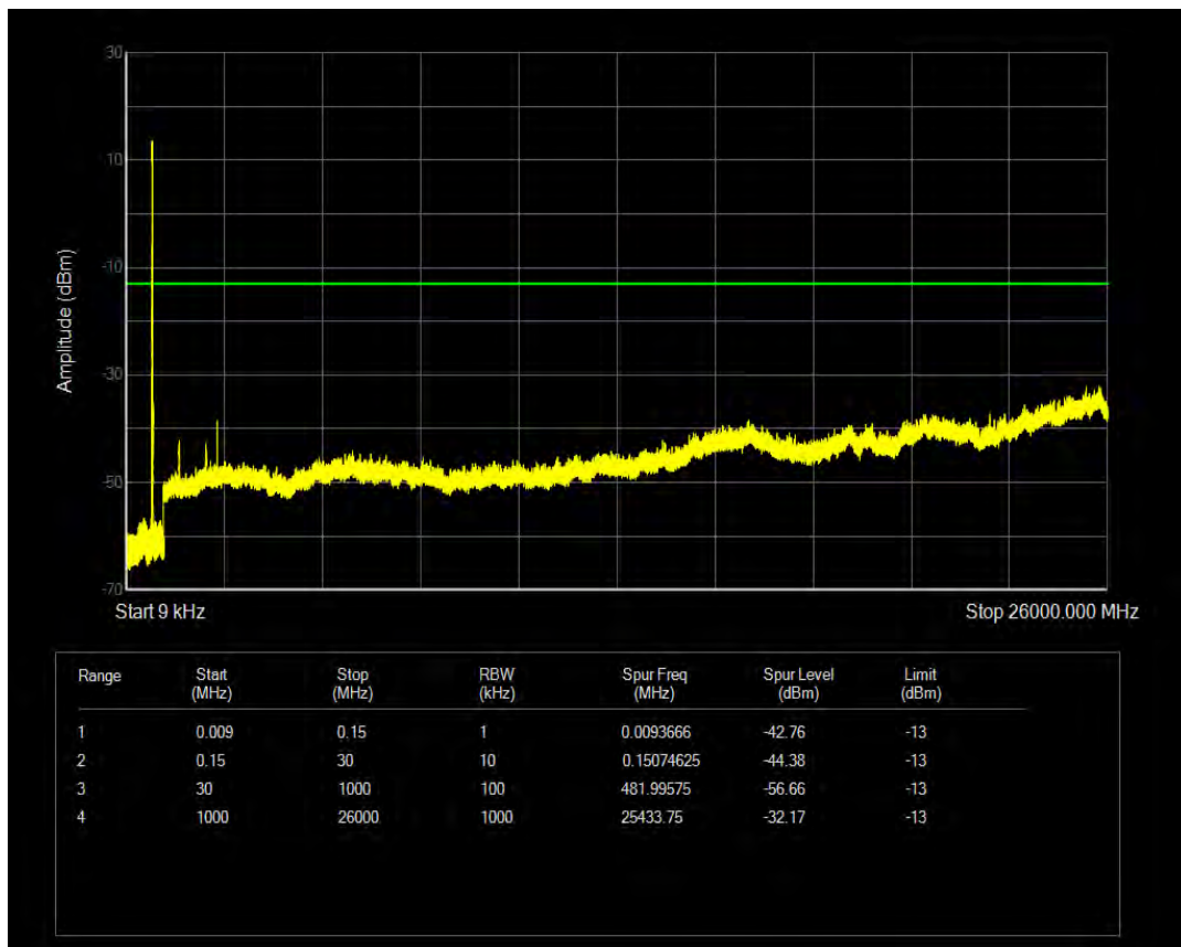
Band17 QAM16 BW=10MHz Channel=23780 RB Size=27 Position=#0
