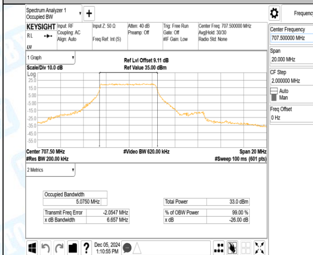
Band12-10MHz-16QAM-23095-27RB#0-PASS
