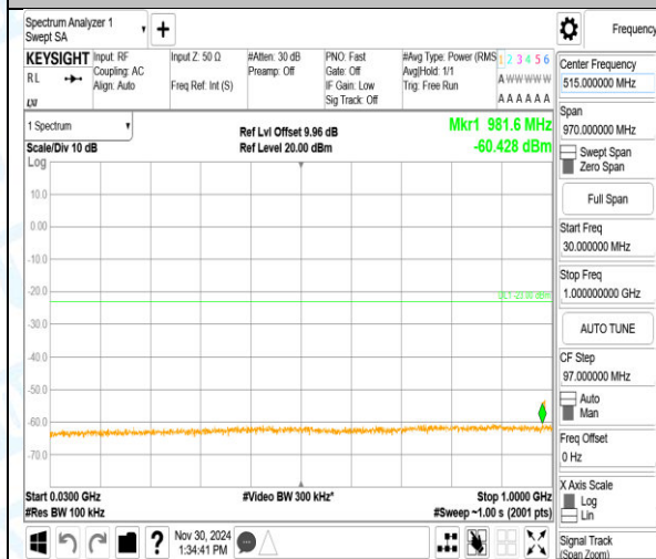
Band4_5MHz_QPSK_19975_1RB#0_3000~20000_3000~20000
