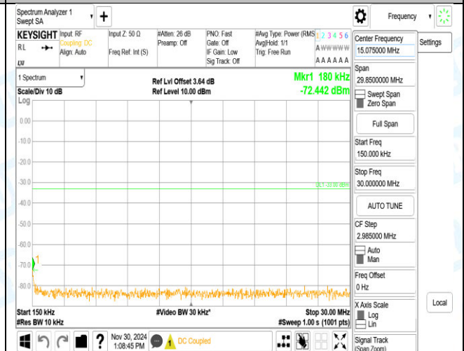
Band4_3MHz_16QAM_20175_15RB#0_1000~3000_1000~3000
