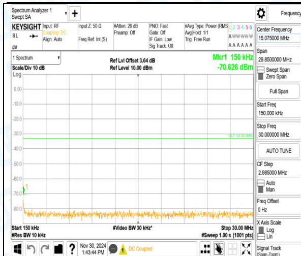
Band4_5MHz_16QAM_20175_1RB#24_1000~3000_1000~3000
