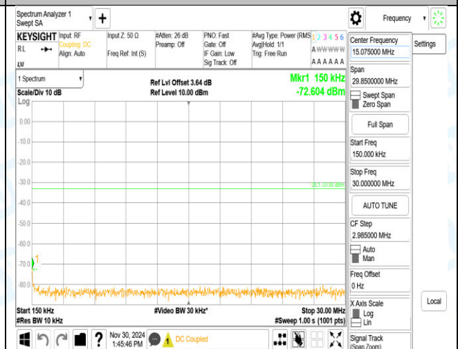
Band4_5MHz_16QAM_20175_25RB#0_1000~3000_1000~3000
