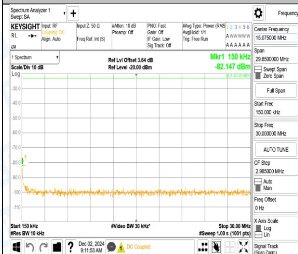
Band5_1.4MHz_QPSK_20525_1RB#0_1000~3000_1000~3000
