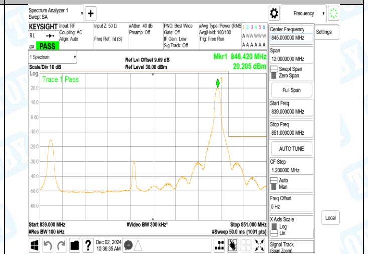
Band5_10MHz_16QAM_20600_1RB#49
