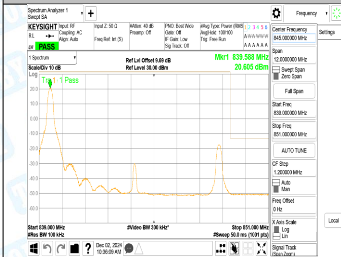
Band5_10MHz_16QAM_20600_1RB#0
