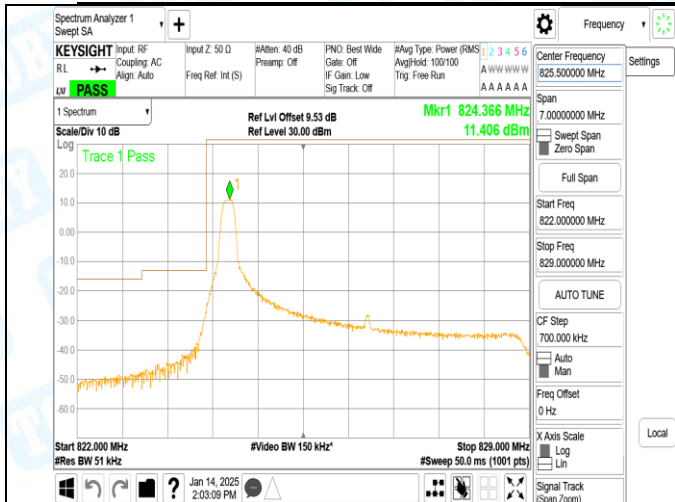
Band5_5MHz_16QAM_20425_25RB#0
