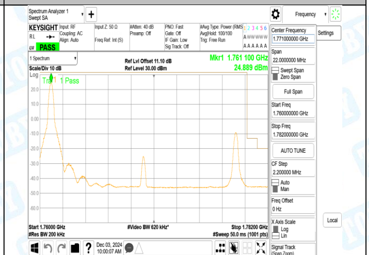
Band66_20MHz_QPSK_132572_100RB#0
