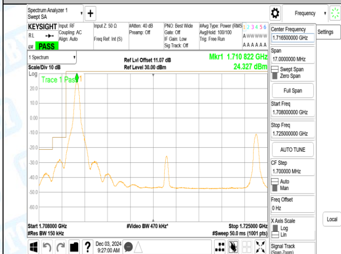
Band66_15MHz_QPSK_132047_75RB#0
