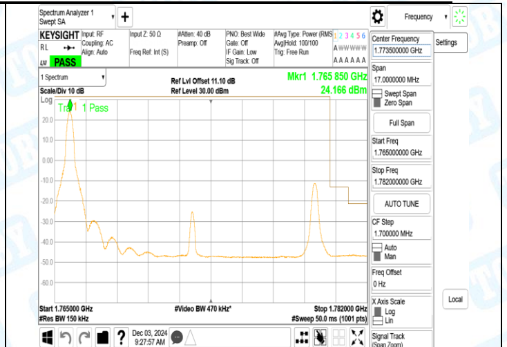
Band66_15MHz_QPSK_132597_75RB#0
