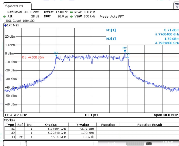
11A-Ant1-5785-PASS
