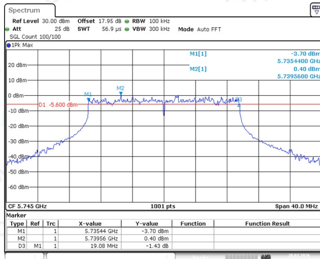
11AX20SISO-Ant1-5745-PASS
