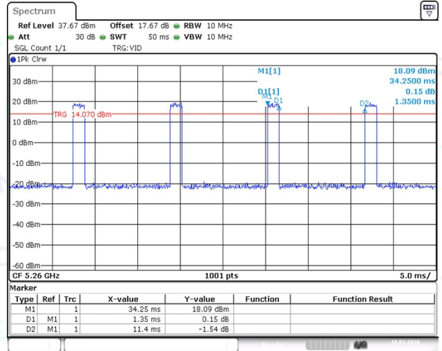
NTNV-11A-Ant1-5260
