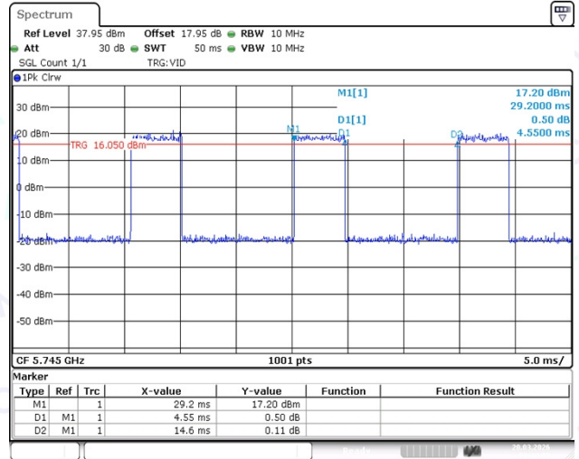
NTVN-11N20SISO-Ant1-5745
