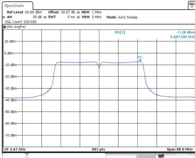
11N40SISO-Ant1-5670-PASS
