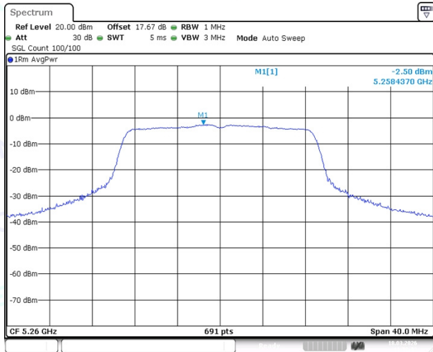
11AC20SISO-Ant1-5260-PASS
