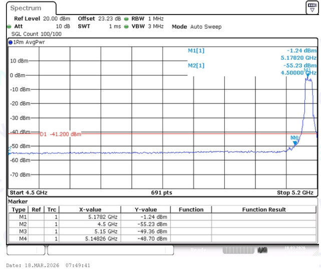
11A-Ant1-5180-PASS
