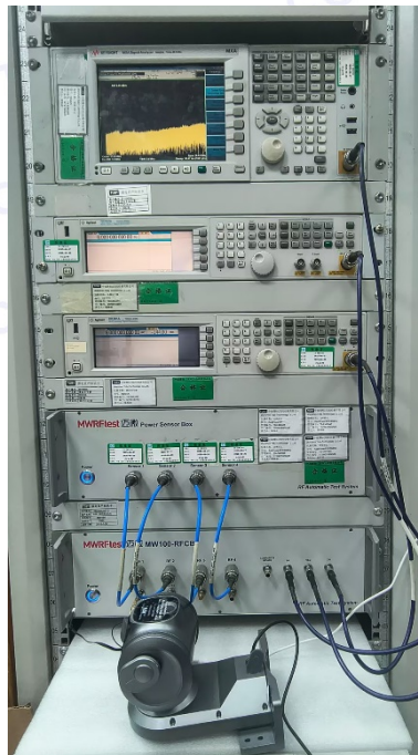
Photo of Setup for Conducted Measurements
