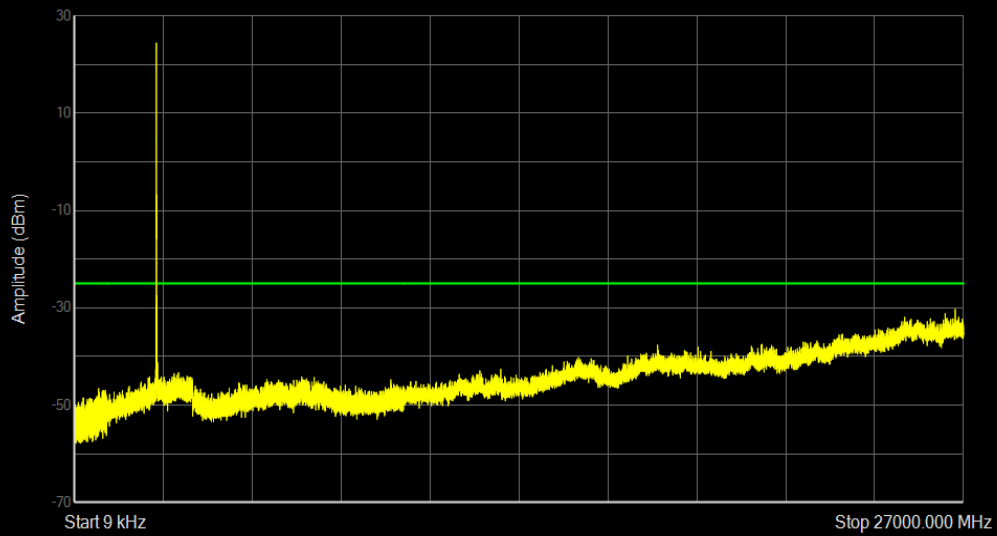
Band7 16QAM BW=10MHz Channel=20800 RB Size=1 Position=#0
