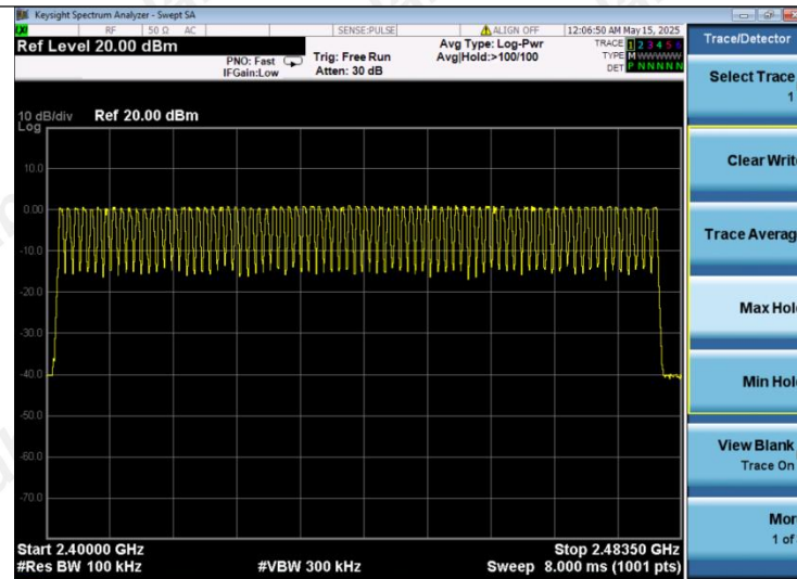
GFSK Modulation
