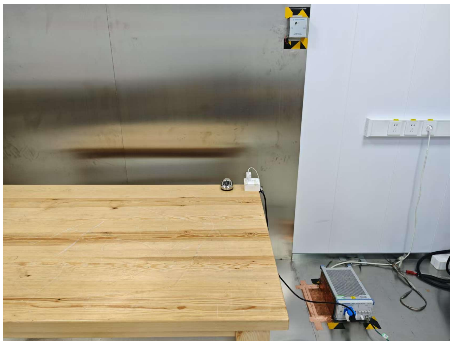
Conducted Emission View
