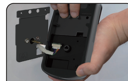
Step4 Connect the cable
