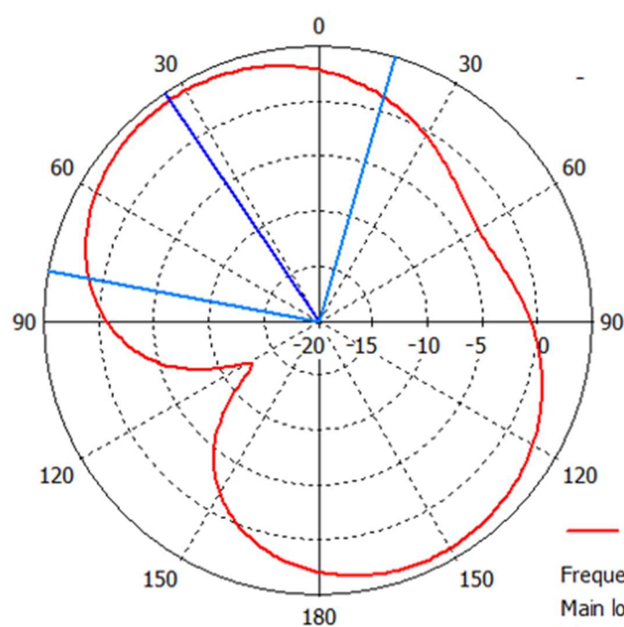
Farfield Gain Abs (Phi=0)
