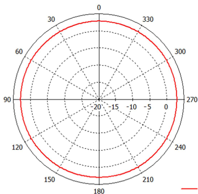
Farfield Gain Abs (Theta=0)
