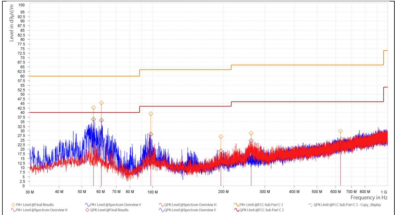
30 MHz – 1 GHz
