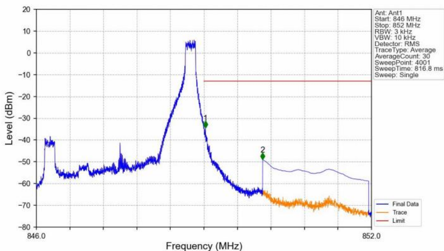
Band5_3MHz_16QAM_HCH_847.5MHz_RB_1_14_NTNV
