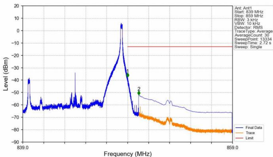
Band5 10MHz 16QAM HCH 844MHz RB 1 49 NTV
