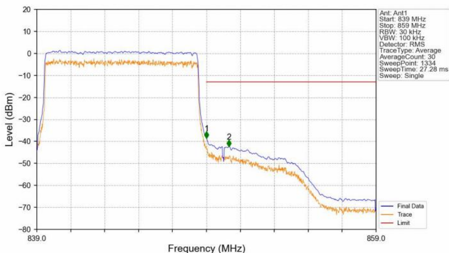
Band5 10MHz 16QAM HCH 844MHz RB 50 0 NTV
