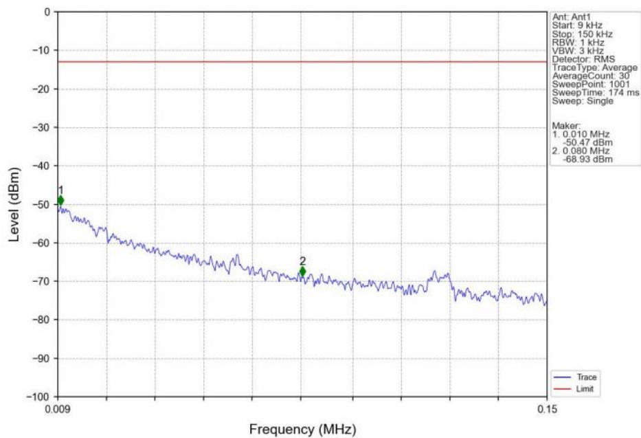
Band5 3MHz 16QAM LCH 825.5MHz RB 1 0 NTNV
