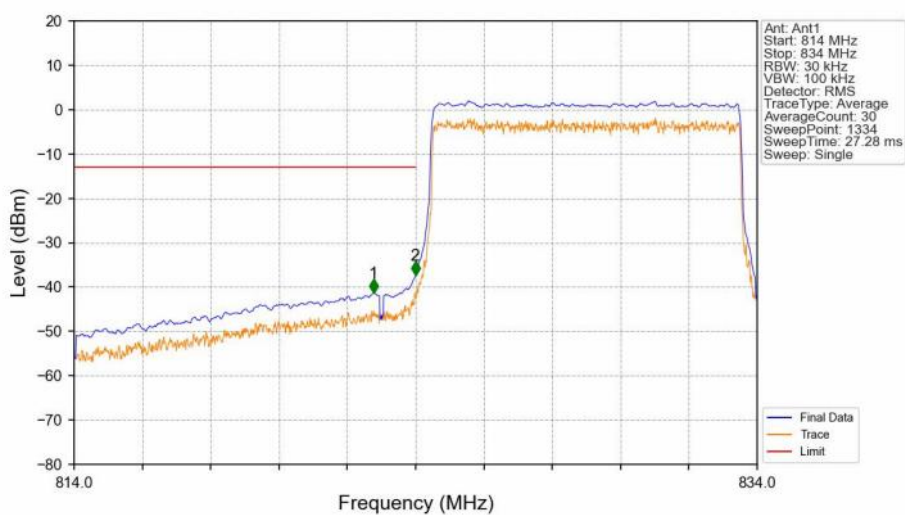
Band5_10MHz_16QAM_LCH_829MHz_RB_50_0_NTNV
