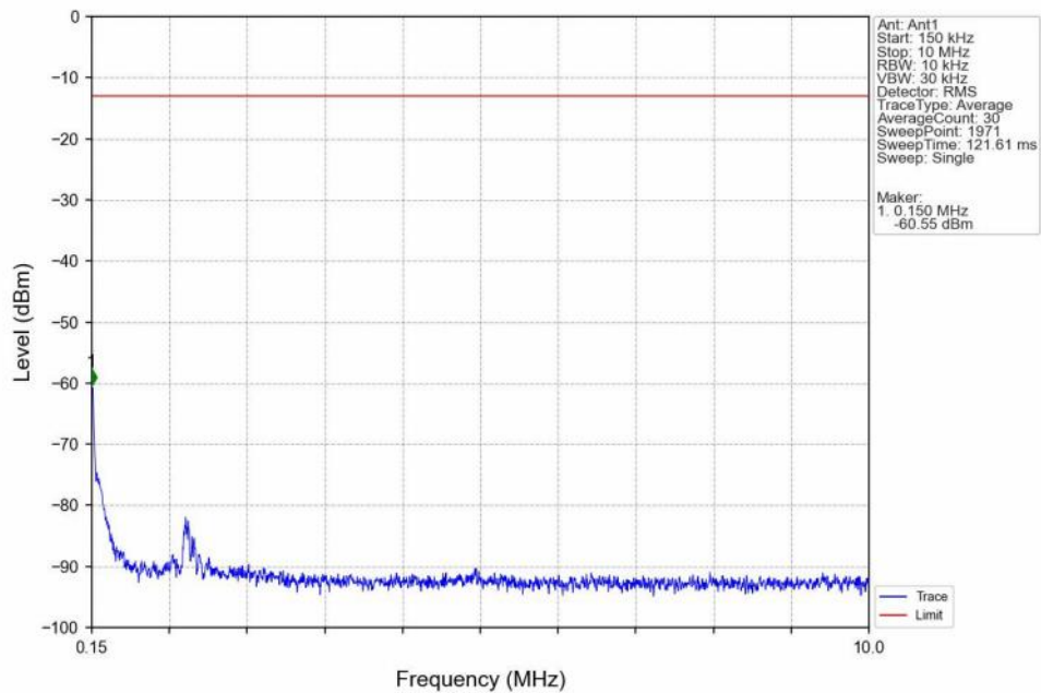
Band66_3MHz_QPSK_HCH_1778.5MHz_RB_1_0_NTNV
