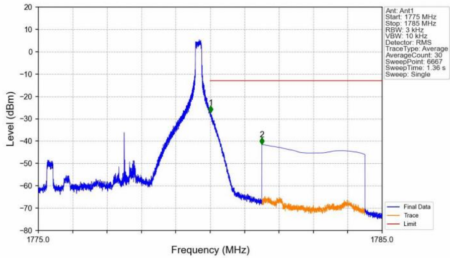
Band66_5MHz_16QAM_HCH_1777.5MHz_RB_1_24_NTNV
