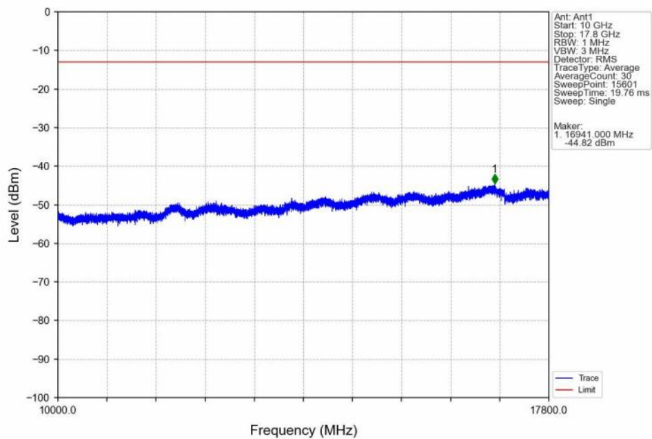
Band66_3MHz_QPSK_LCH_1711.5MHz_RB_1_0_NTNV
