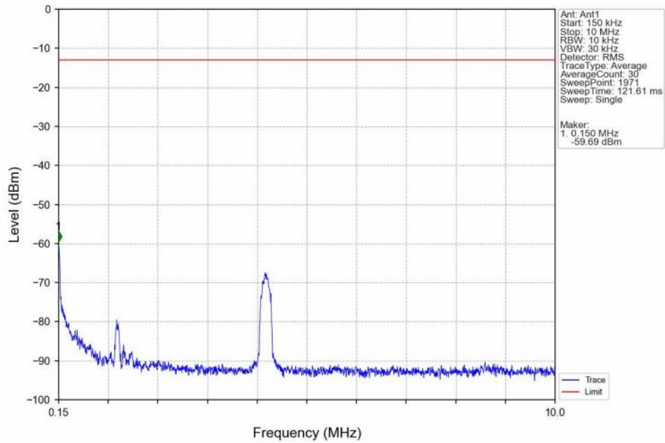
Band66_5MHz_QPSK_LCH_1712.5MHz_RB_1_0_NTNV
