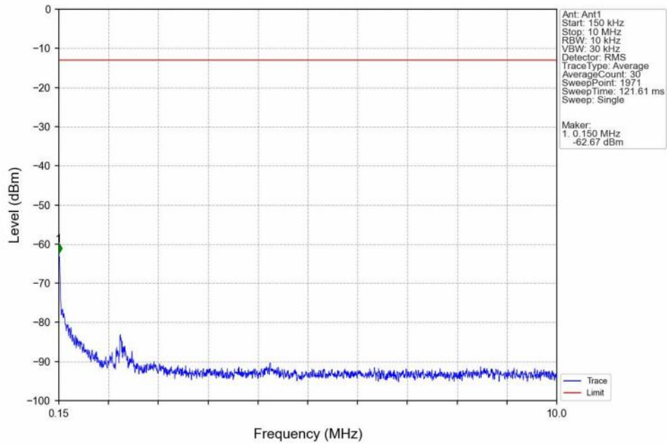
Band66_5MHz_16QAM_HCH_1777.5MHz_RB_1_0_NTNV
