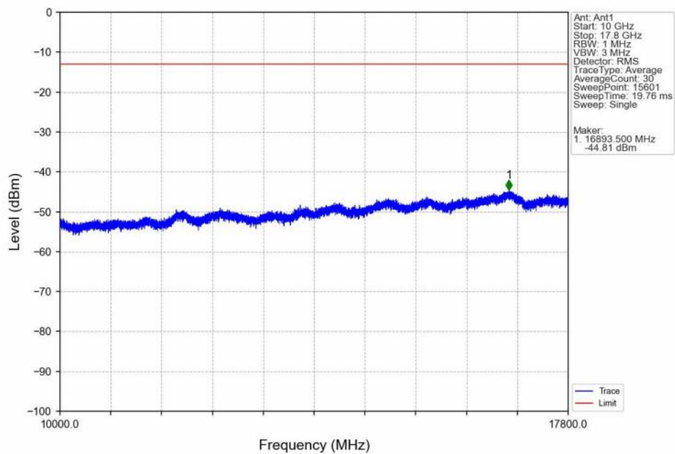
Band66_5MHz_QPSK_LCH_1712.5MHz_RB_1_0_NTNV
