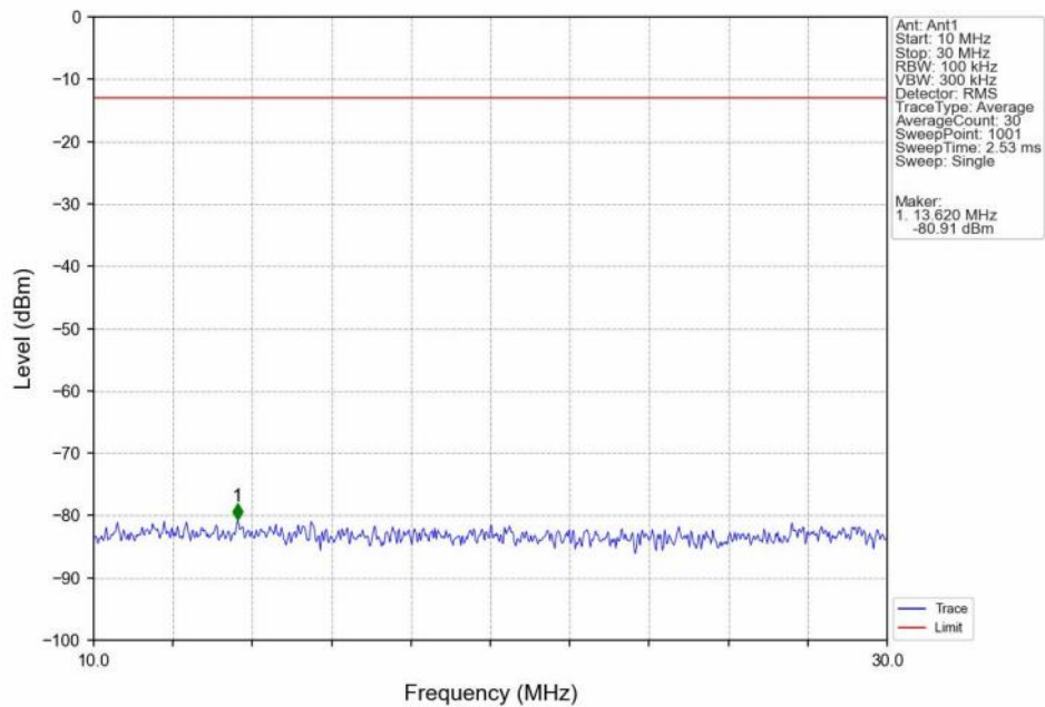
Band5 HSUPA LCH 826.4MHz Subtest 1 NTN
