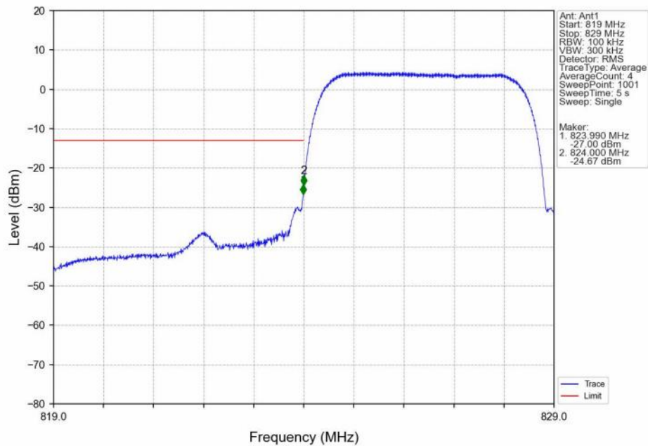
Band5 HSUPA LCH 826.4MHz Subtest 1 NTN
