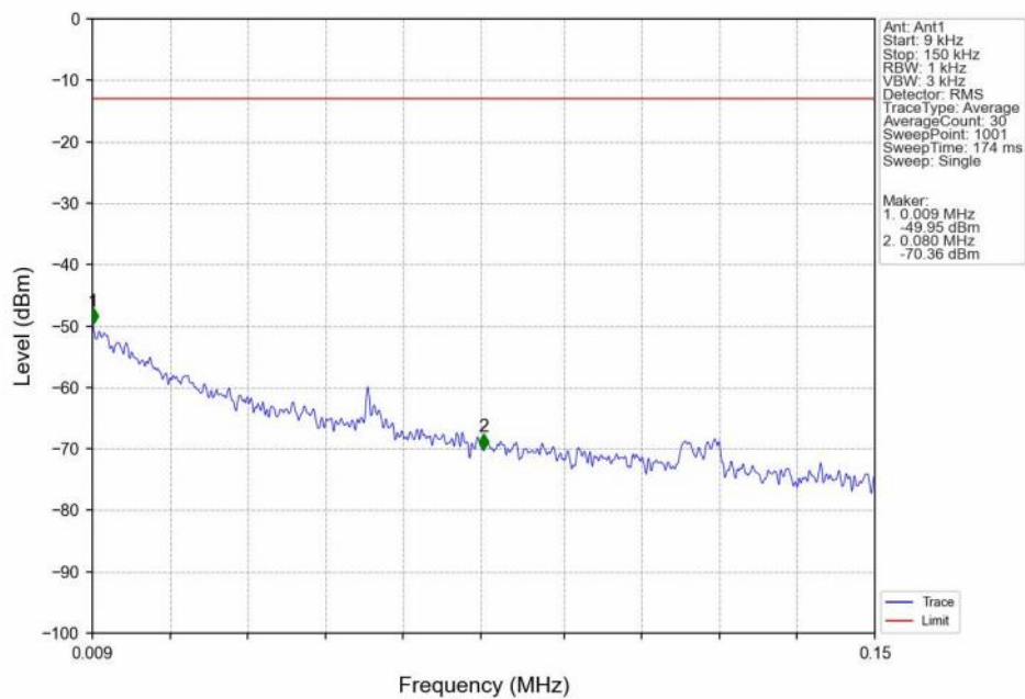
Band5 HSUPA LCH 826.4MHz Subtest 1 NTN
