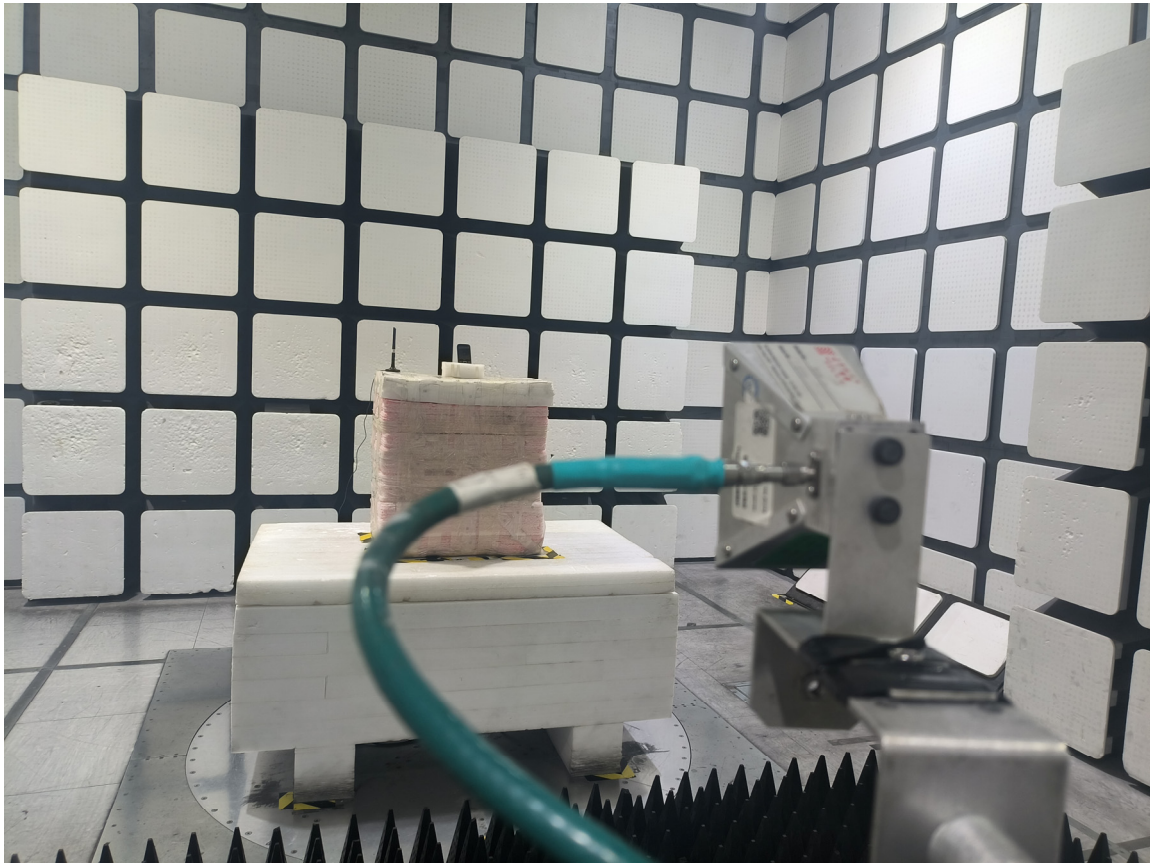
Radiated Emissions View (18-27 GHz)
