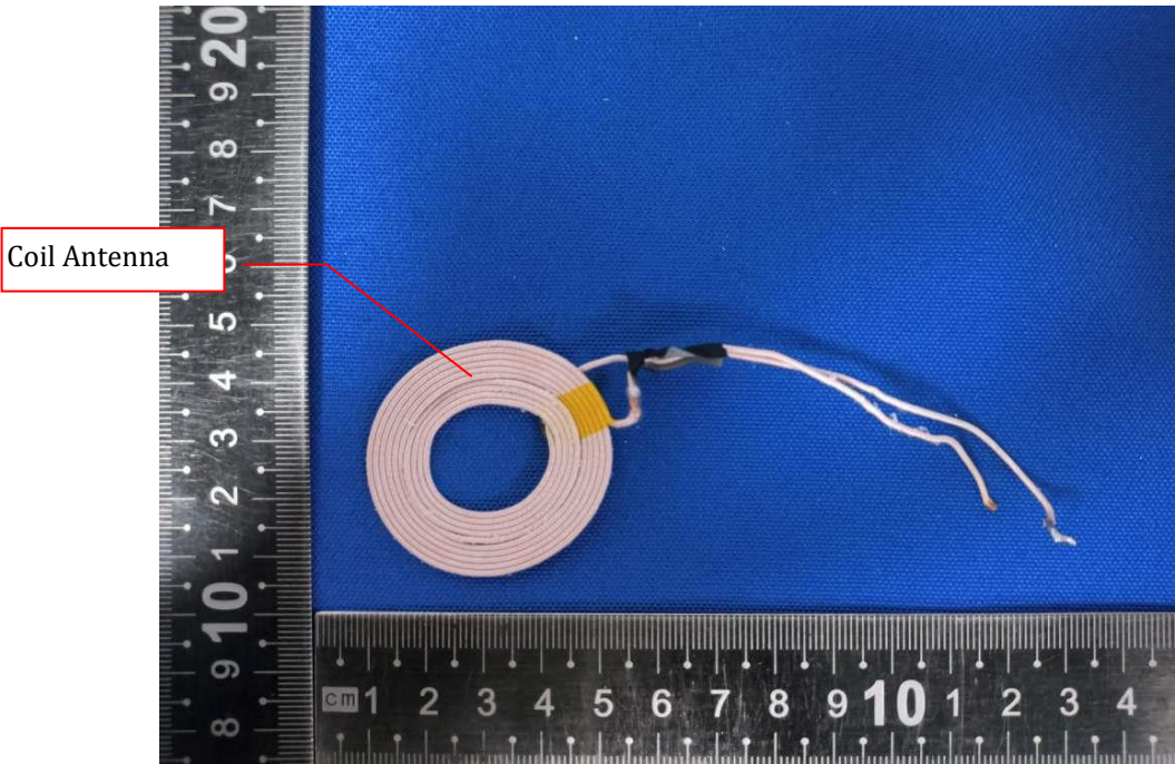
EUT Internal View 8
