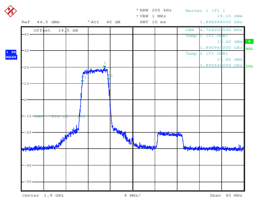
Occupied Bandwidth
