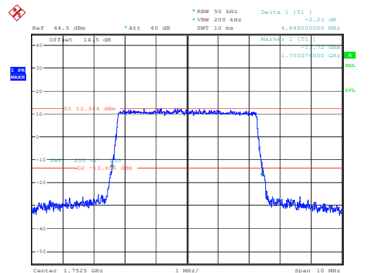
26dB Bandwidth
