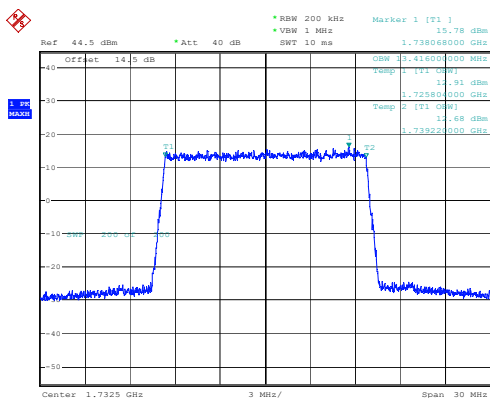
Occupied Bandwidth
