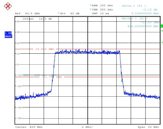
26dB Bandwidth
