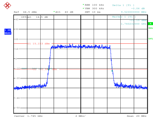
26dB Bandwidth
