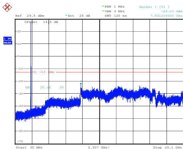
20MHz_Middle_QPSK_1@0(30MHz~20.1GHz)
