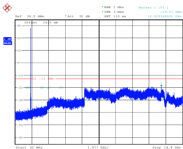
15MHz_Middle_QPSK_1@0(30MHz~18.8GHz)
