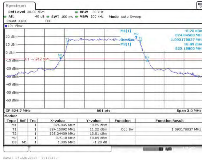
Band5-1.4MHz-QPSK-20525-6RB#0
