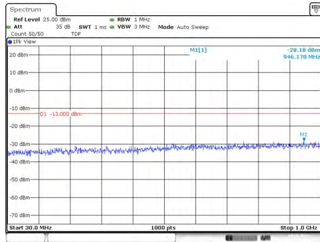
Band2-1.4MHz-QPSK-18607-6RB#0-Range1:30~1000MHz
