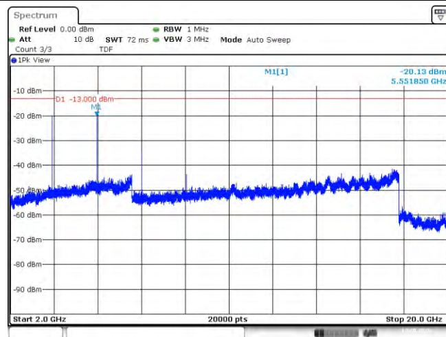
Band2-1.4MHz-QPSK-18607-6RB#0-Range3:2000~20000MHz
