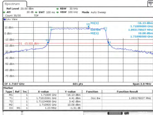
Band66-1.4MHz-QPSK-131979-6RB#0-1.093
