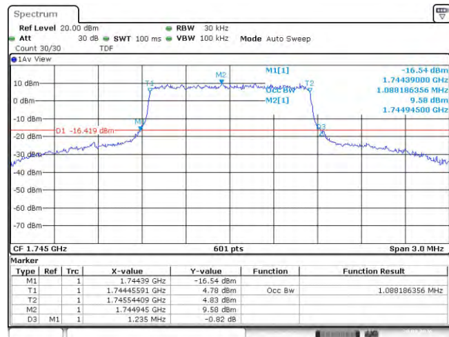
Band66-1.4MHz-QPSK-132322-6RB#0-1.088
