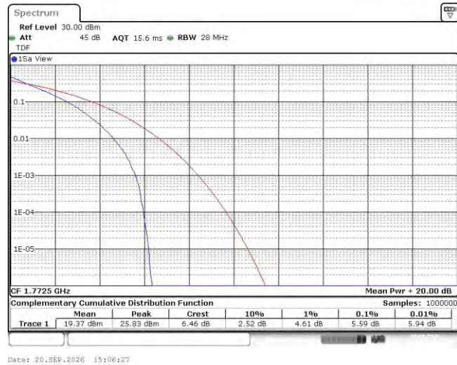
Band66-15MHz-16QAM-132047-1RB#0
