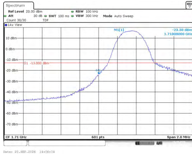
Band66-5MHz-16QAM-131997-1RB#24
