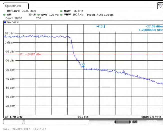
Band66-3MHz-QPSK-131987-1RB#0
