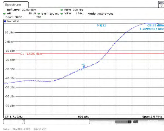
Band66-15MHz-QPSK-132047-1RB#74
