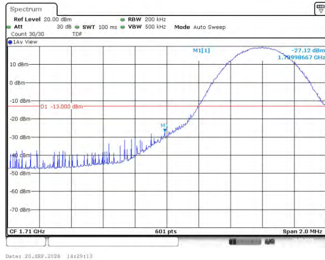
Band66-10MHz-16QAM-132022-1RB#49
