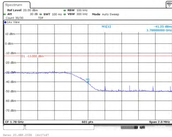
Band66-5MHz-QPSK-132647-1RB#24
