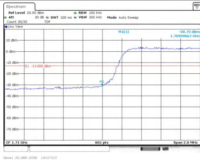
Band66-5MHz-QPSK-132647-1RB#0
