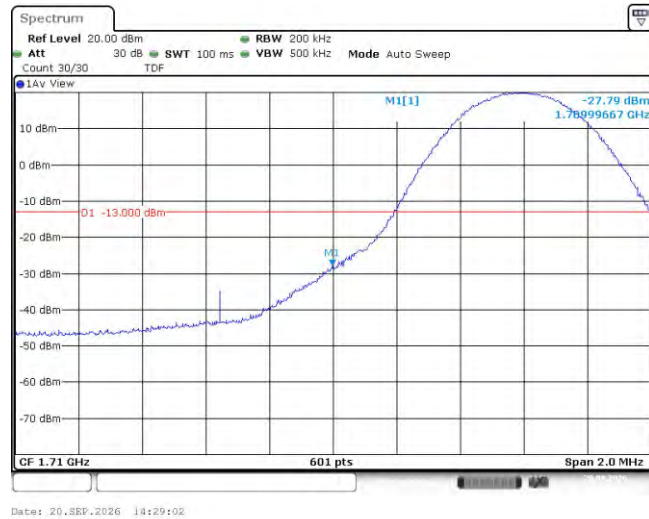
Band66-10MHz-QPSK-132022-1RB#49
