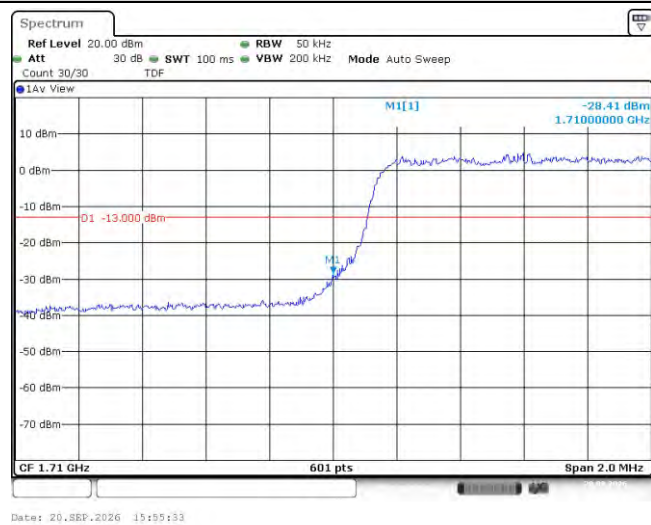
Band66-3MHz-16QAM-132657-1RB#0
