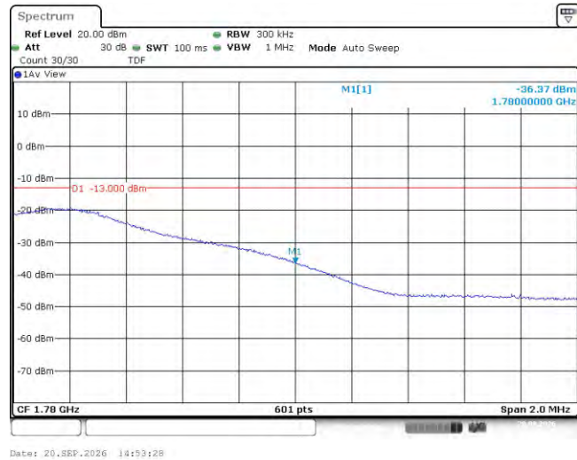
Band66-15MHz-QPSK-132597-1RB#74
