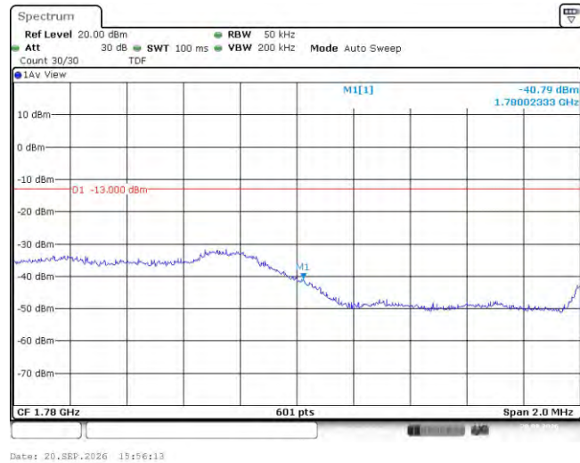
Band66-3MHz-16QAM-132657-1RB#14
