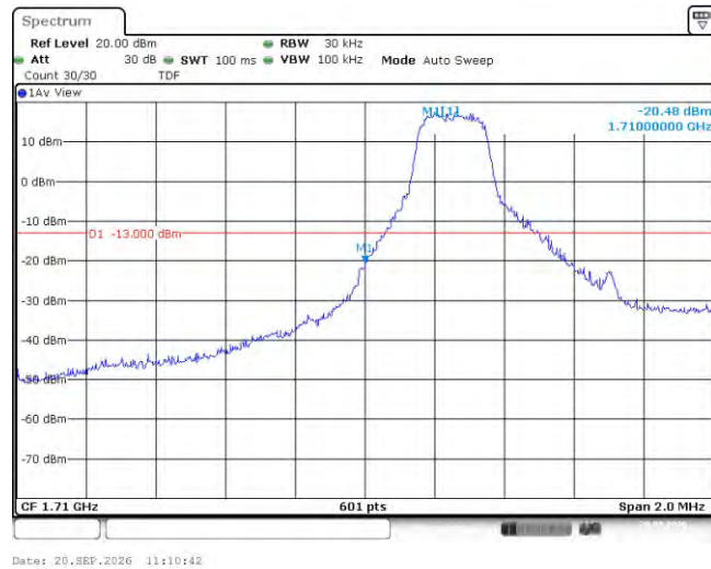
Band66-1.4MHz-QPSK-131979-1RB#5
