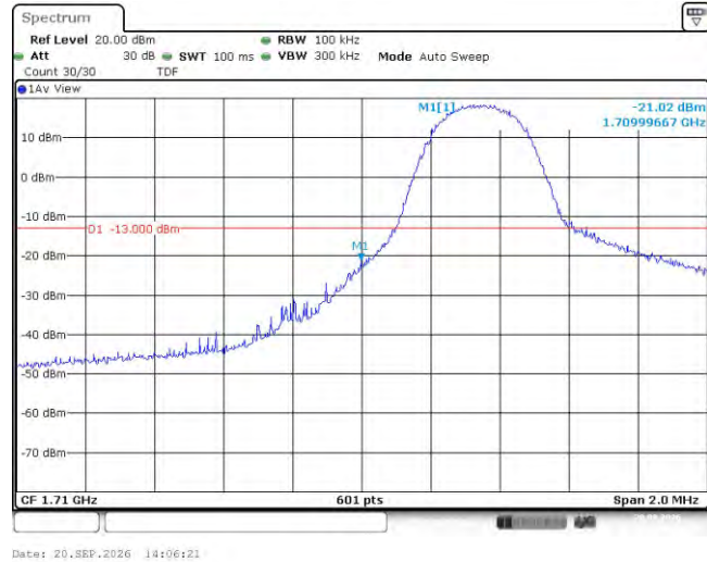
Band66-5MHz-QPSK-131997-1RB#24
