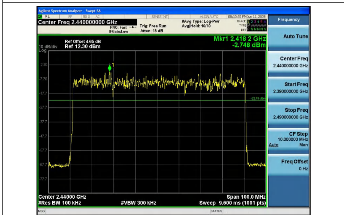
2_Band_Edge_(Hopping)_NVNT_ANT1_3-DH5_Hopping
