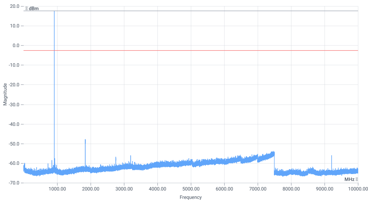
TX emissions
