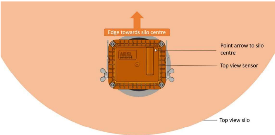
Figure 9: Sensor orientation
