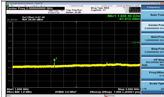
Band5_5MHz_16QAM_20425_25RB#0_1000~3000_1000 ~3000
