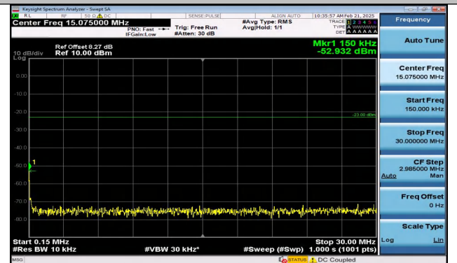
Band5_5MHz_QPSK_20525_1RB#0_0.15~30_0.15~30
