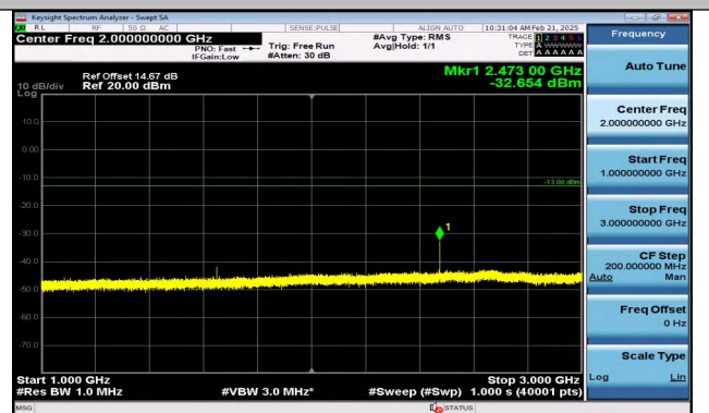
Band5_5MHz_QPSK_20425_1RB#0_1000~3000_1000~3000
