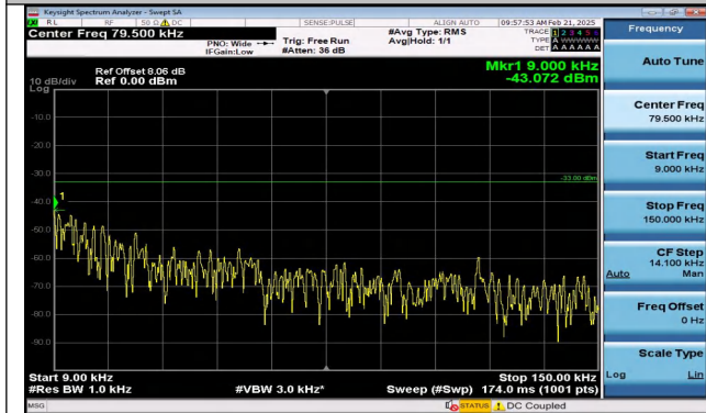
Band5_3MHz_QPSK_20635_1RB#0_0.009~0.15_0.009~0.15 .15
