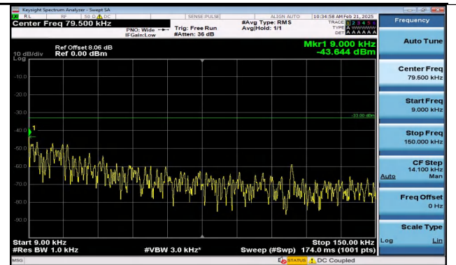
Band5_5MHz_16QAM_20425_25RB#0_0.009~0.15_0.009 ~0.15
