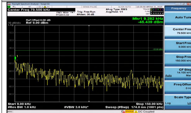
Band5_5MHz_QPSK_20525_1RB#0_0.009~0.15_0.009~0 .15
