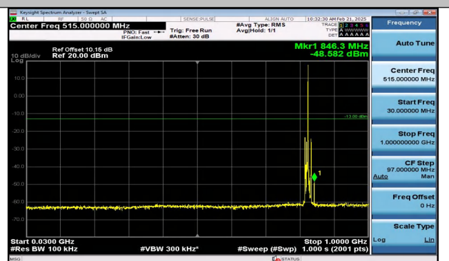
Band5_5MHz_QPSK_20425_1RB#24_30~1000_30~1000
