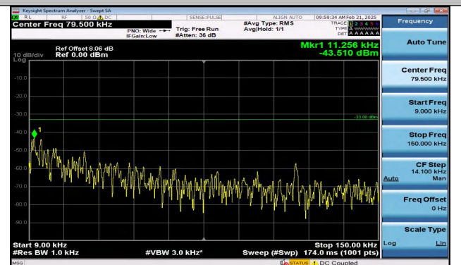
Band5_3MHz_QPSK_20635_1RB#14_0.009~0.15_0.009~0.15 0.15
