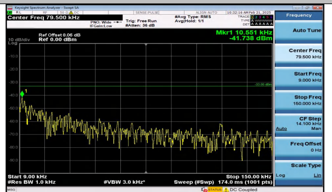
Band5_5MHz_QPSK_20425_1RB#24_0.009~0.15_0.009~0.15
