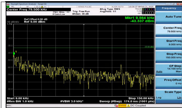
Band5_5MHz_QPSK_20425_1RB#0_0.009~0.15_0.009~0.15
