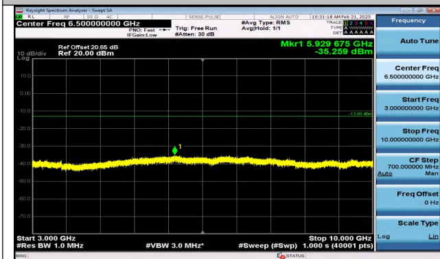
Band5_5MHz_QPSK_20425_1RB#0_3000~10000_3000~10000
