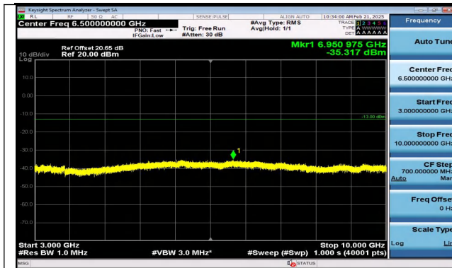
Band5_5MHz_16QAM_20425_1RB#24_3000~10000_300 0~10000
