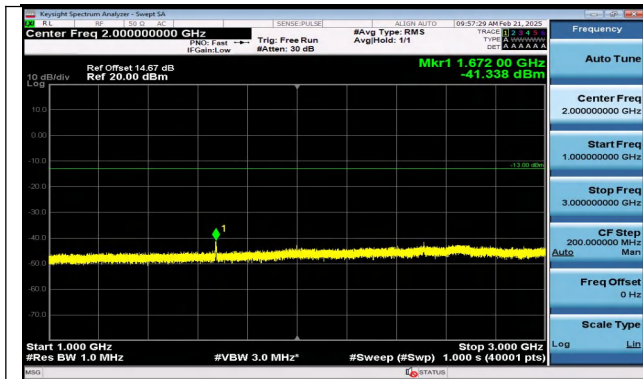
Band5_3MHz_16QAM_20525_15RB#0_1000~3000_1000 ~3000
