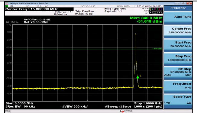
Band5_5MHz_16QAM_20425_25RB#0_30~1000_30~100 0
