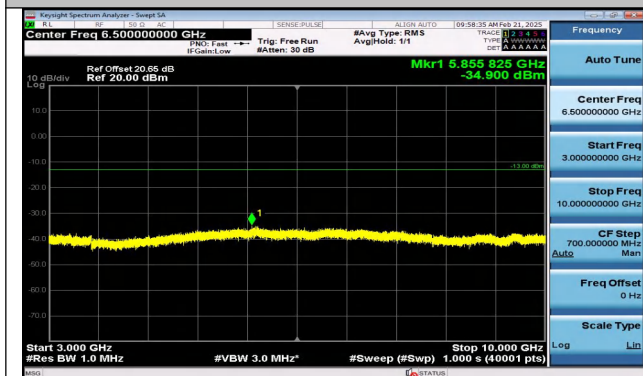
Band5_3MHz_QPSK_20635_1RB#0_3000~10000_3000~10000 10000
