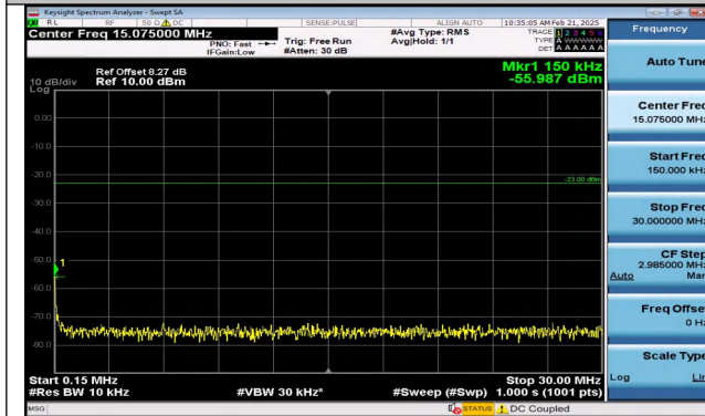
Band5_5MHz_16QAM_20425_25RB#0_0.15~30_0.15~30
