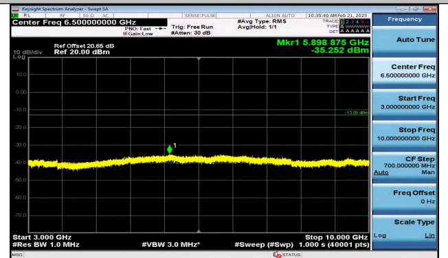
Band5_5MHz_16QAM_20425_25RB#0_3000~10000_300 0~10000
