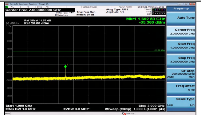
Band5_3MHz_QPSK_20635_1RB#0_1000~3000_1000~3000 000
