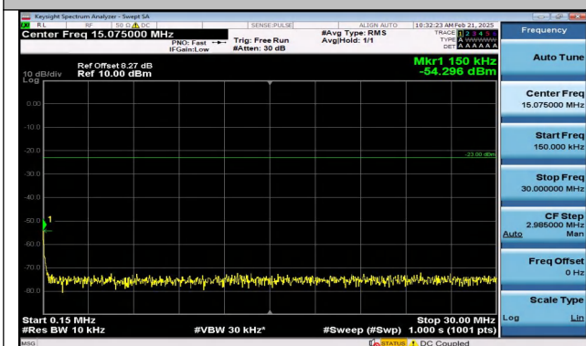
Band5_5MHz_QPSK_20425_1RB#24_0.15~30_0.15~30
