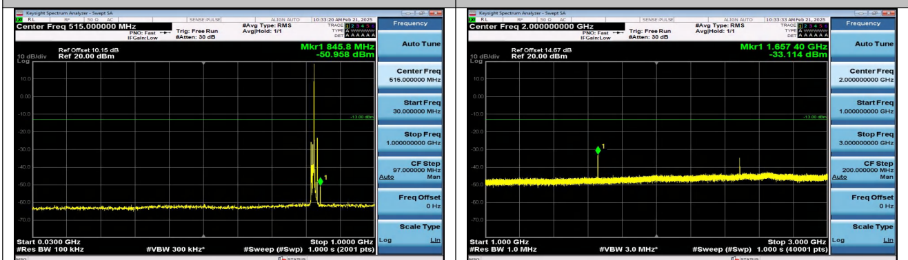
Band5_5MHz_16QAM_20425_1RB#24_30~1000_30~1000
