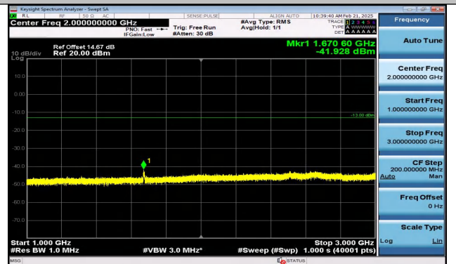
Band5_5MHz_QPSK_20525_25RB#0_1000~3000_1000~3000
