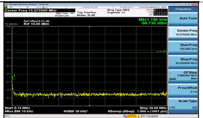
Band5_5MHz_16QAM_20625_1RB#24_0.15~30_0.15~30
