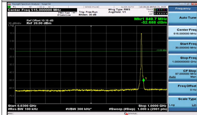
Band5_5MHz_QPSK_20525_25RB#0_30~1000_30~1000
