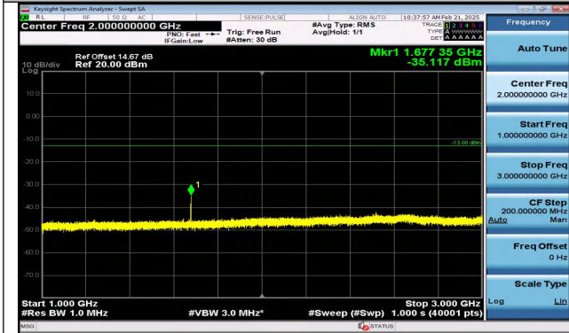
Band5_5MHz_QPSK_20525_1RB#24_1000~3000_1000~3000
