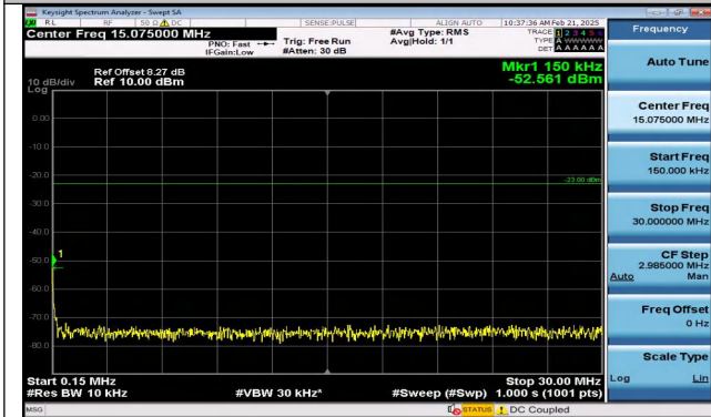
Band5_5MHz_QPSK_20525_1RB#24_0.15~30_0.15~30
