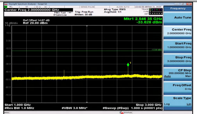
Band5_5MHz_16QAM_20625_1RB#24_1000~3000_1000 ~3000
