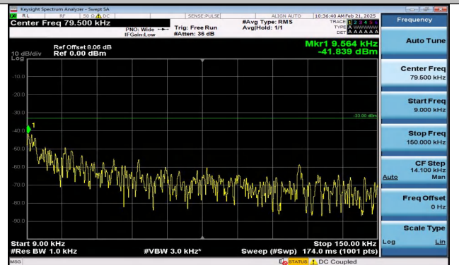
Band5_5MHz_16QAM_20525_1RB#0_0.009~0.15_0.009~0.15
