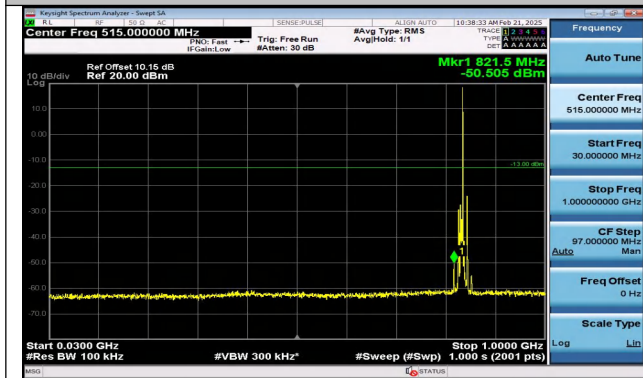
Band5_5MHz_16QAM_20525_1RB#24_30~1000_30~1000
