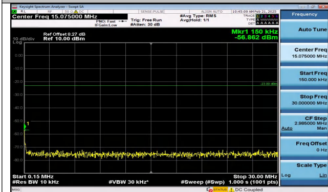
Band5_5MHz_16QAM_20625_25RB#0_0.15~30_0.15~30
