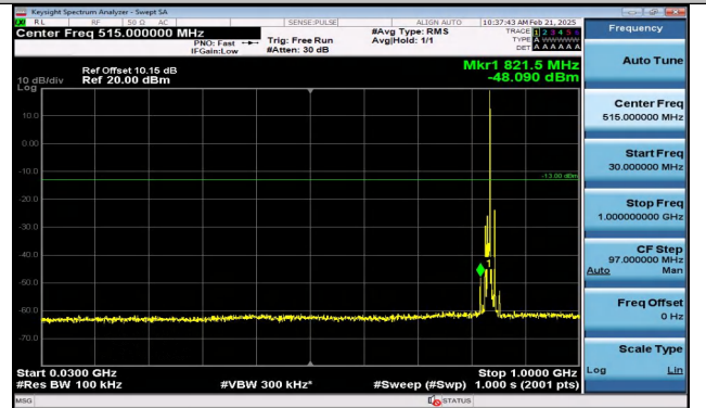
Band5_5MHz_QPSK_20525_1RB#24_30~1000_30~1000
