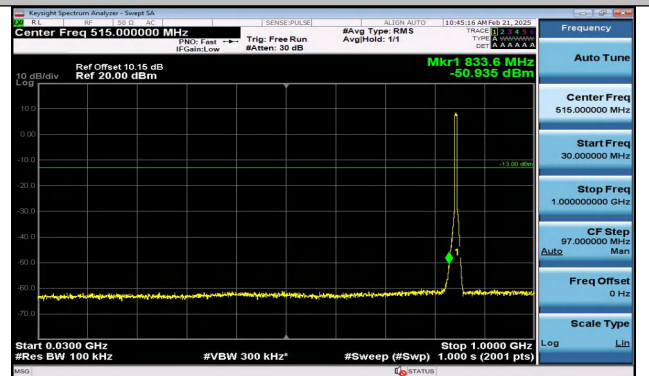
Band5_5MHz_16QAM_20625_25RB#0_30~1000_30~100 0
