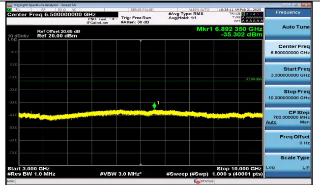
Band5_5MHz_QPSK_20525_1RB#24_3000~10000_3000~10000
