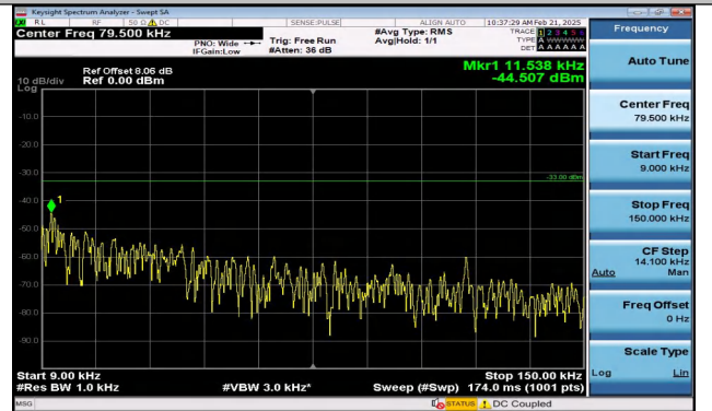
Band5_5MHz_QPSK_20525_1RB#24_0.009~0.15_0.009~0.15
