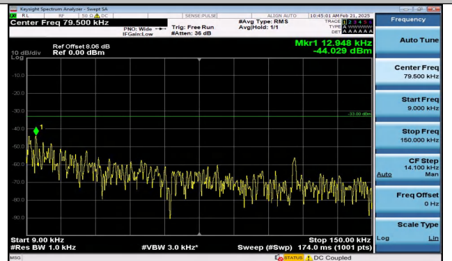
Band5_5MHz_16QAM_20625_25RB#0_0.009~0.15_0.009 ~0.15
