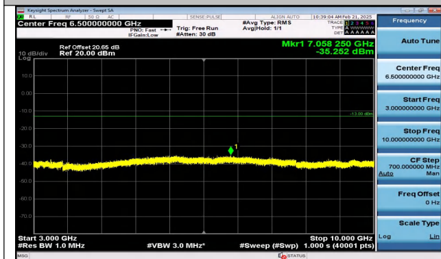
Band5_5MHz_16QAM_20525_1RB#24_3000~10000_3000~10000
