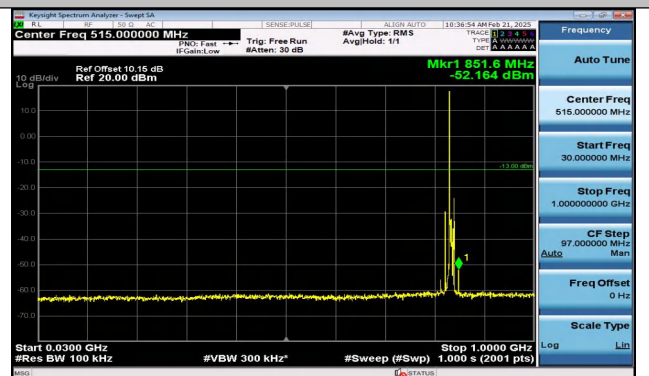
Band5_5MHz_16QAM_20525_1RB#0_30~1000_30~1000
