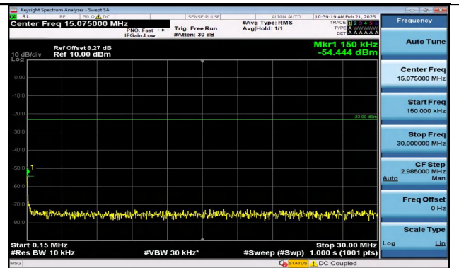
Band5_5MHz_QPSK_20525_25RB#0_0.15~30_0.15~30
