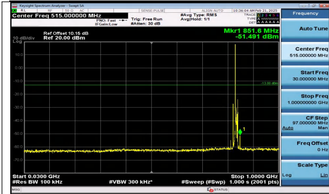
Band5_5MHz_QPSK_20525_1RB#0_30~1000_30~1000
