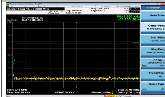
Band5_5MHz_16QAM_20525_1RB#0_0.15~30_0.15~30
