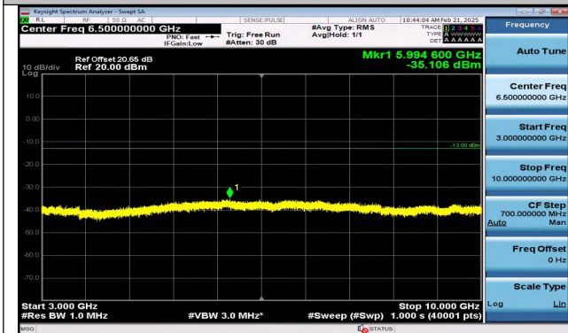
Band5_5MHz_16QAM_20625_1RB#24_3000~10000_300 0~10000
