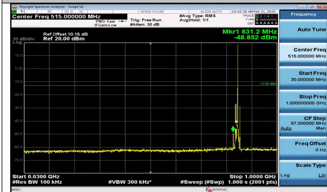
Band5_5MHz_16QAM_20625_1RB#24_30~1000_30~100 0
