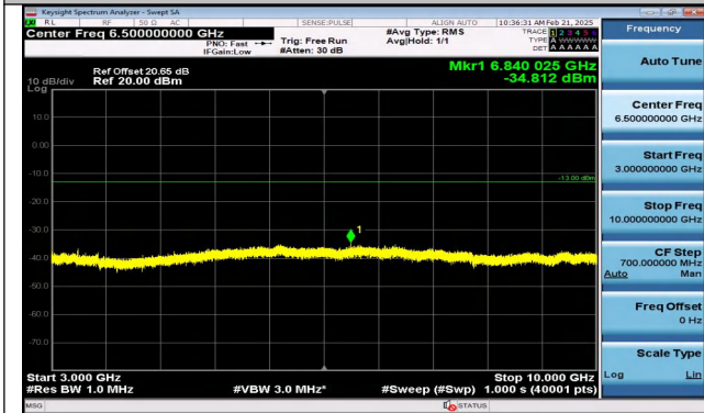
Band5_5MHz_QPSK_20525_1RB#0_3000~10000_3000~10000
