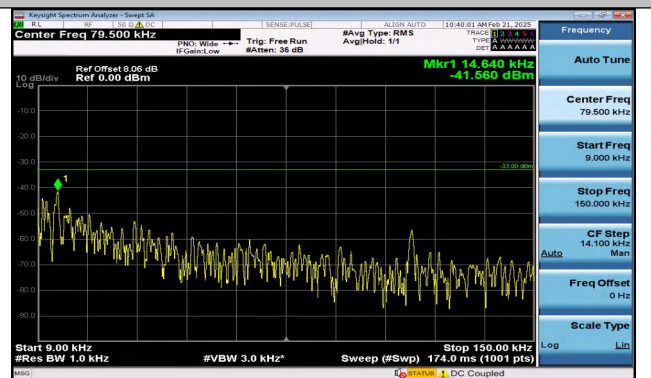
Band5_5MHz_16QAM_20525_25RB#0_0.009~0.15_0.009~0.15
