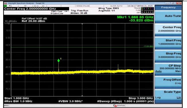
Band5_5MHz_QPSK_20525_1RB#0_1000~3000_1000~3000
