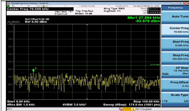
Band7_15MHz_16QAM_21375_1RB#0_0.009~0.15_0.009~0.15
