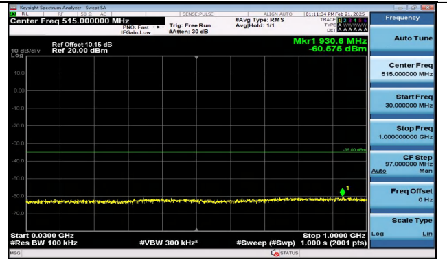
Band7_15MHz_QPSK_21375_75RB#0_30~1000_30~1000
