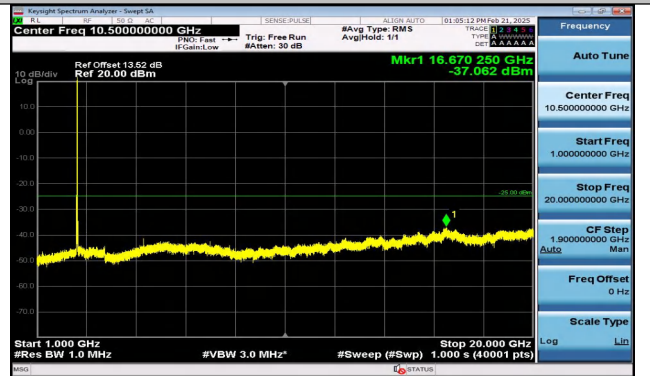
Band7_15MHz_16QAM_21100_1RB#74_1000~20000_10 00~20000
