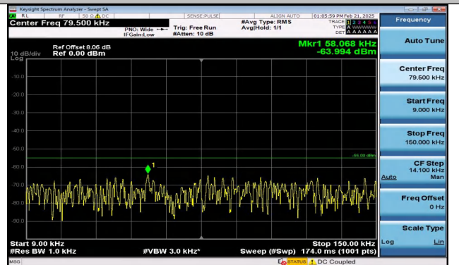
Band7_15MHz_QPSK_21375_1RB#0_0.009~0.15_0.009~0.15 0.15
