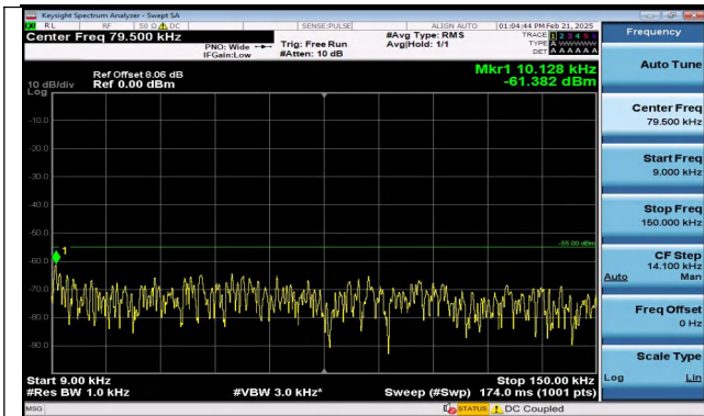
Band7_15MHz_16QAM_21100_1RB#74_0.009~0.15_0.00 9~0.15
