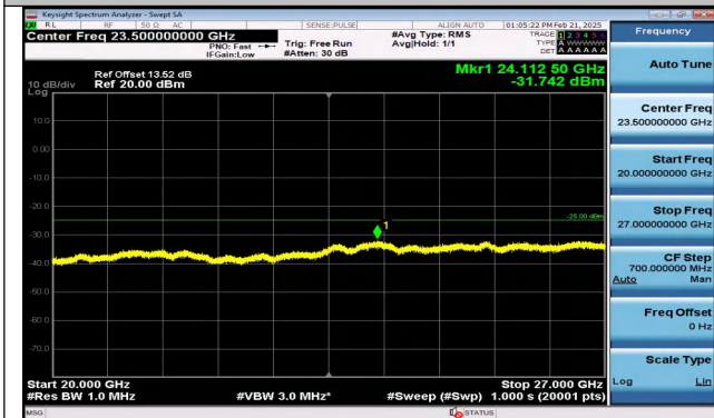
Band7_15MHz_16QAM_21100_1RB#74_20000~27000_2 0000~27000
