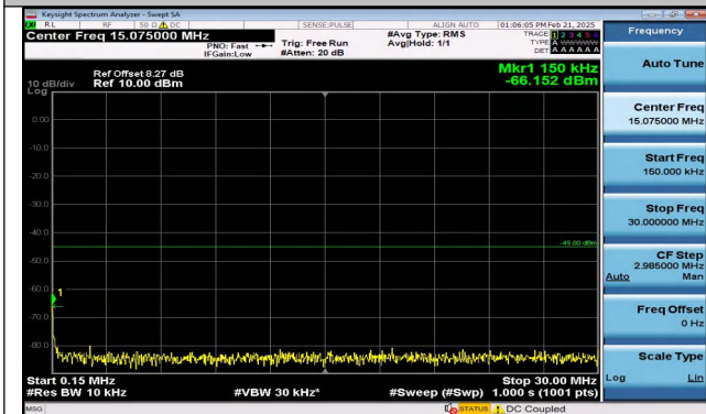
Band7_15MHz_QPSK_21375_1RB#0_0.15~30_0.15~30
