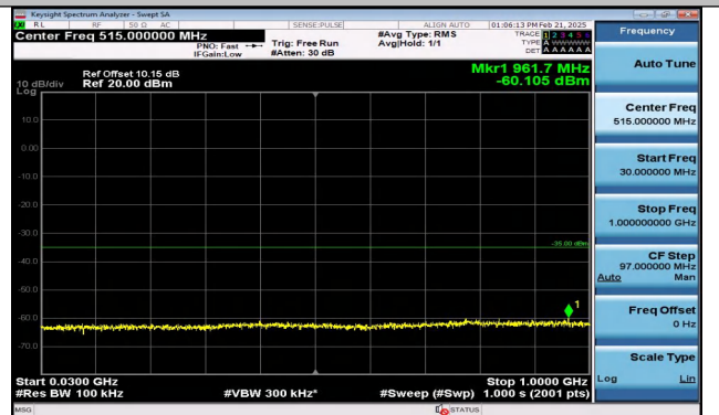
Band7_15MHz_QPSK_21375_1RB#0_30~1000_30~1000
