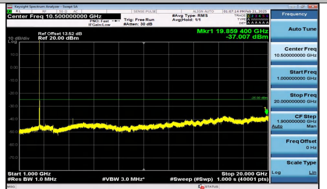
Band7_15MHz_16QAM_21375_1RB#0_1000~20000_1000~20000
