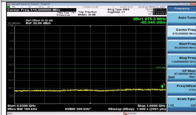
Band7_15MHz_16QAM_21375_1RB#0_30~1000_30~1000
