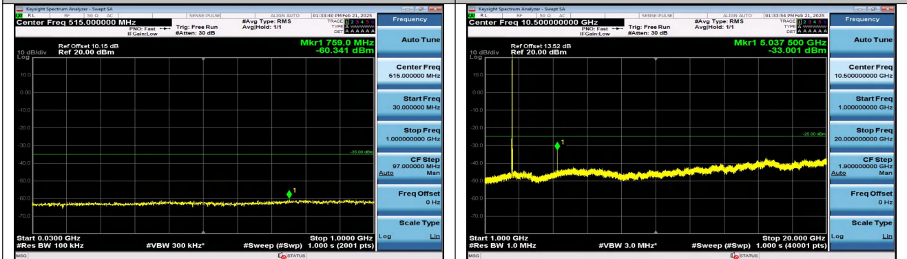
Band7_20MHz_16QAM_20850_1RB#99_30~1000_30~10 00
