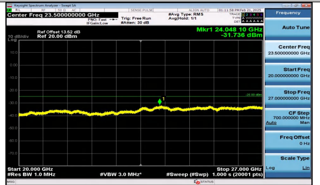
Band7_15MHz_QPSK_21375_75RB#0_20000~27000_20000~27000
