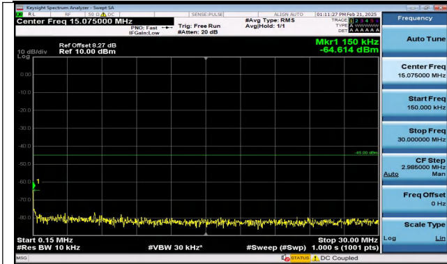
Band7_15MHz_QPSK_21375_75RB#0_0.15~30_0.15~30
