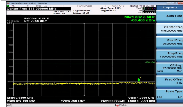
Band7_15MHz_16QAM_21100_1RB#74_30~1000_30~10 00
