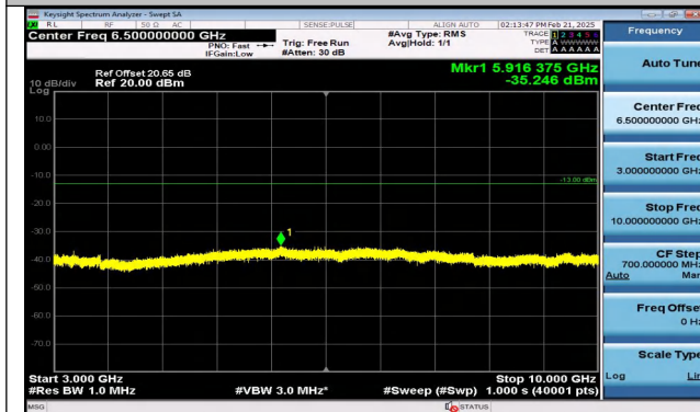
Band12_1.4MHz_QPSK_23173_1RB#0_3000~10000_300 0~10000
