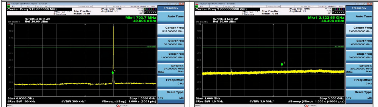
Band12_1.4MHz_QPSK_23095_6RB#0_30~1000_30~1000
