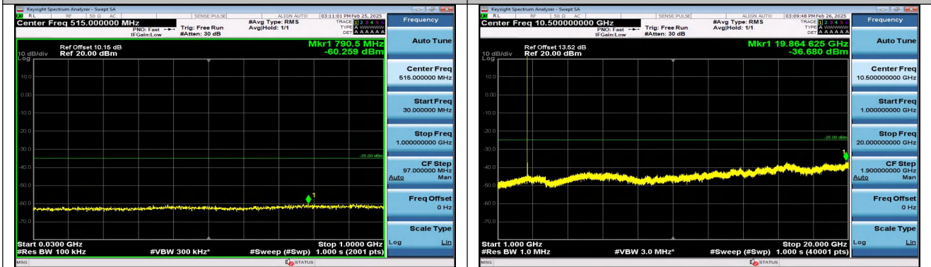
Band41_15MHz_16QAM_40620_1RB#74_30~1000_30~1 000
