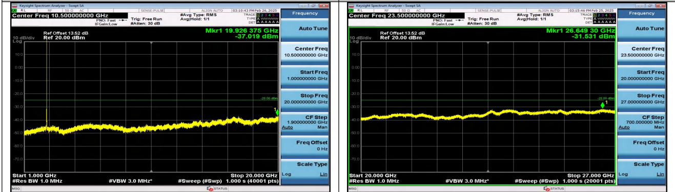
Band41_15MHz_16QAM_41515_1RB#74_1000~20000_1 000~20000
