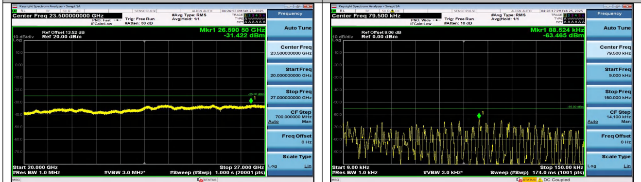
Band41_20MHz_16QAM_39750_1RB#99_20000~27000_20000~27000
