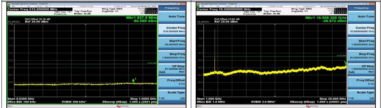
Band41_20MHz_QPSK_39750_100RB#0_30~1000_30~1 000
