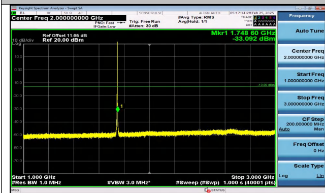
Band66_1.4MHz_16QAM_132322_6RB#0_1000~3000_10 00~3000
