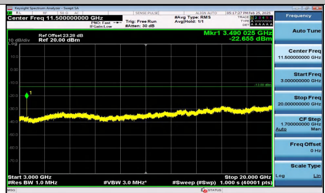
Band66_1.4MHz_16QAM_132322_6RB#0_3000~20000_3 000~20000
