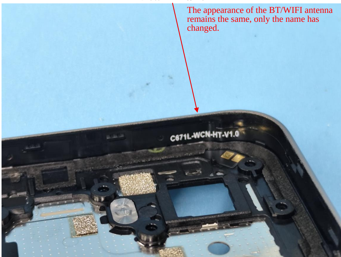
BT/Wi-Fi Antenna
